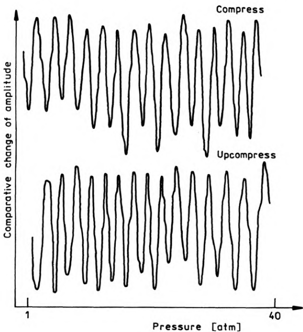
Fig. 7. Result of measurement of pressure sensitivity. The length of optical fibre was 1 m. The pressure was changed with the range 0.1–4 MPa. The pressure sensitivity is 24 rad/MPam
