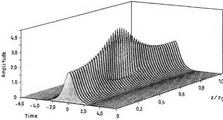
Fig. 1. Evolution of the second order soliton
