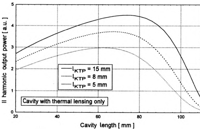
Fig. 3. Dependence of II harmonic output power on cavity length for pump power of 15 W and several lengths of KTP crystal.
