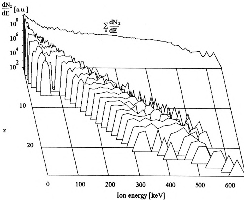
Fig. 4. Energy distribution of Ta ions species estimated on the basis of the IEA signals measured at different deflecting potentials (different E_i/z ratios).
