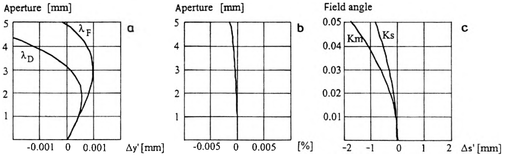
Fig. 7. Hybrid lens E: a – transversal spherical aberration, b – deviation from the sine condition, c – field curvature.
