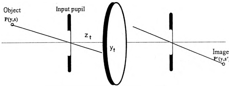
Fig. 10. Hybrid lens with shifted entrance pupil.
