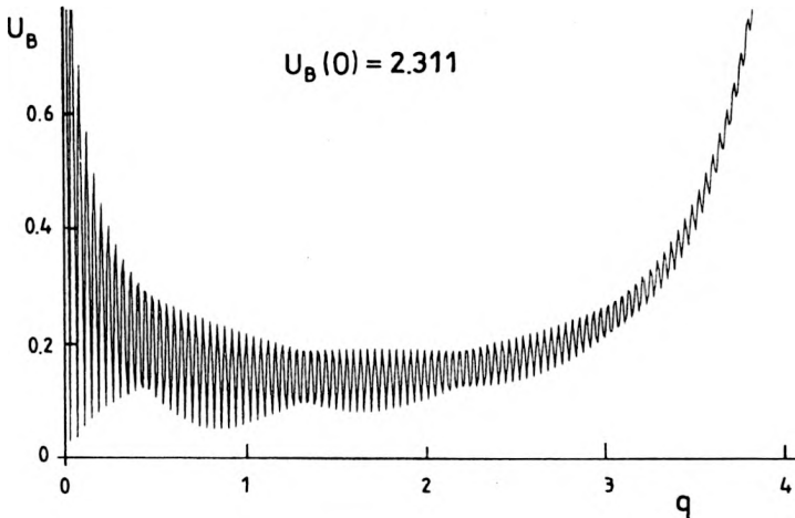
Fig. 1. Boundary diffraction wave amplitude vs. radial distance in observation plane for the filter designed according to relation (2). Filter function has radial symmetry and its derivative at the edge equals zero.
