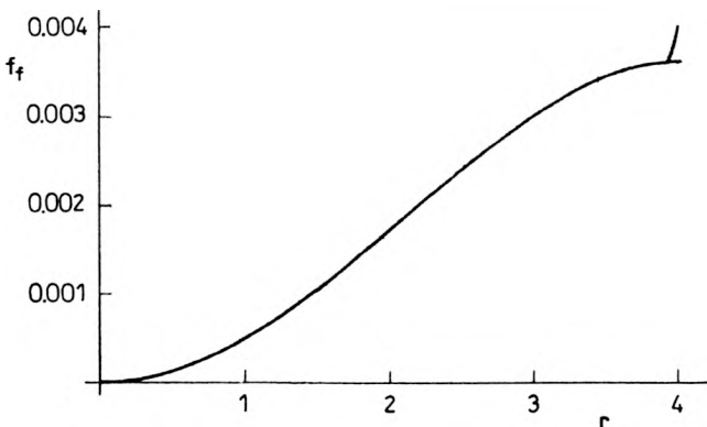
Fig. 2. Filter function obtained from relation (2) with the condition (5) which should assure a uniform intensity distribution and a filter extension according to relation (6).
