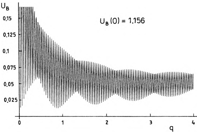
Fig. 3. Boundary diffraction wave amplitude vs. observation point position for the filter which behaving radial symmetry is modified at the edge according to relation (6). We observe diminution of the amplitude with respect to that of Fig. 1, but in the central part of the observation plane the amplitude, although gets reduced, still remains high.
