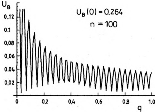
Fig. 4. Boundary diffraction wave amplitude vs. observation point position lying in the meridional plane, for the filter whose function was modified at the edge introducing angular derivative according to relation (7) in order to diminish the amplitude value in the central part of the observation plane. The quoted results are limited to 0 \leq r \leq 1 for the reason of time-consuming calculations.
