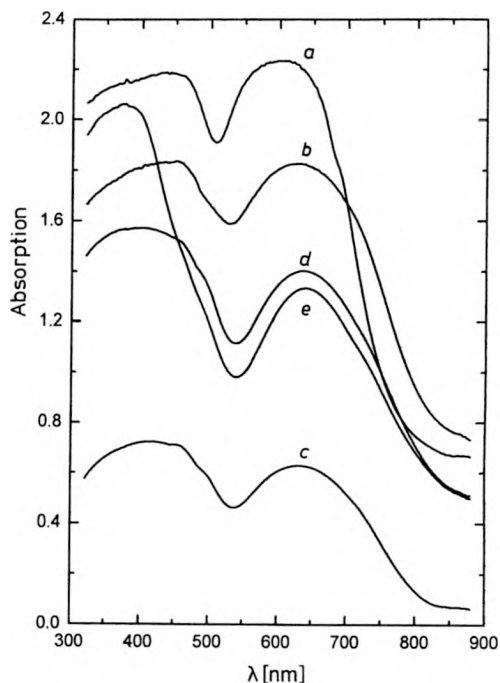
Fig. 3. UV-Vis absorption spectra of xerogels of the type \text{SiO}_2\text{-TiO}_2 : 100 \text{SiO}_2 (a), 75 \text{SiO}_2\text{-25TiO}_2 (b), 50 \text{SiO}_2\text{-50TiO}_2 (c), 25 \text{SiO}_2\text{-75TiO}_2 (d), 100 \text{TiO}_2 (e), in mol%, doped with 3 mol% \text{Cr}^{3+} .
