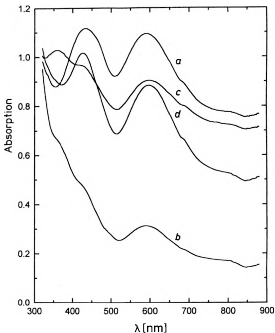
Fig. 1. UV-Vis absorption spectra of xerogels of the type \text{NaO}_2\text{-B}_2\text{O}_3\text{-SiO}_2 : 5.8 \text{Na}_2\text{O} -11.6 \text{B}_2\text{O}_3 -82.6 \text{SiO}_2 (curve a ), 11.6 \text{Na}_2\text{O} -5.8 \text{B}_2\text{O}_3 -82.6 \text{SiO}_2 (curve b ), 12.5 \text{Na}_2\text{O} -12.5 \text{B}_2\text{O}_3 -75.0 \text{SiO}_2 (curve c ), 13.3 \text{Na}_2\text{O} -20.0 \text{B}_2\text{O}_3 -66.7 \text{SiO}_2 (in mol%), doped with 3 mol% \text{Cr}^{3+} .
