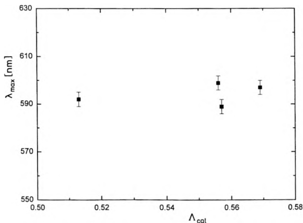
Fig. 2. Variation in the band position \lambda_{\text{max}} (attributed to the {}^4A_{2g} \rightarrow {}^4T_{2g} transition) with calculated optical basicity \Lambda_{\text{cat}} for xerogels of the type \text{Na}_2\text{O-B}_2\text{O}_3\text{-SiO}_2 .
