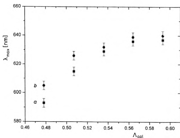
Fig. 4. Variation of the band position \lambda_{\text{max}} (attributed to the {}^4A_{2g} \rightarrow {}^4T_{2g} transition) with calculated optical basicity \Lambda_{\text{cal}} for xerogels of the type \text{SiO}_2\text{-TiO}_2 . The xerogels were dried at 30 °C (a) and 100 °C (b).
