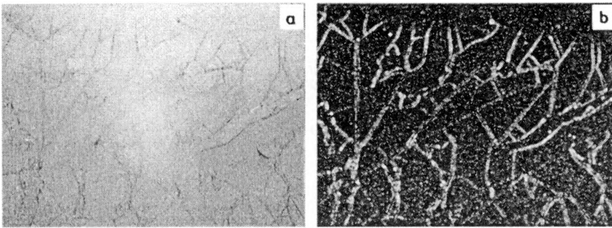
Fig. 6. Microscopic picture (a) of the surface of the sol-gel matrix prepared with the molar ratio R = 15 with water as a solvent and its Sobel transform (b).
