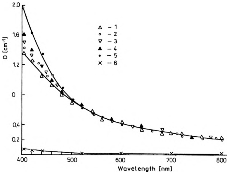
Fig. 1. Spectral dependence of optical density for the porous glass DV-1M after irradiation with \gamma -quanta of ^{60}\text{Co} at different exposure doses: 1 — original glass, 2 — 10^5 R, 3 — 10^6 R, 4 — 10^7 R, 5 — 10^8 R, 6 — the same for the porous glass impregnated with silicon-organic polymer at the \gamma -quanta of ^{60}\text{Co} exposure dose of 10^8 R.
