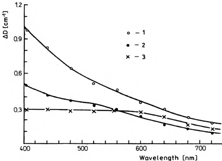
Fig. 2. Spectral dependence of the optical density difference for glasses after irradiation with \gamma -quanta of ^{60}\text{Co} (exposure dose 5 \cdot 10^5 R): 1 — sodium-borate-silicate glass, 2 — quartz-like glass, 3 — melted quartz KU.
