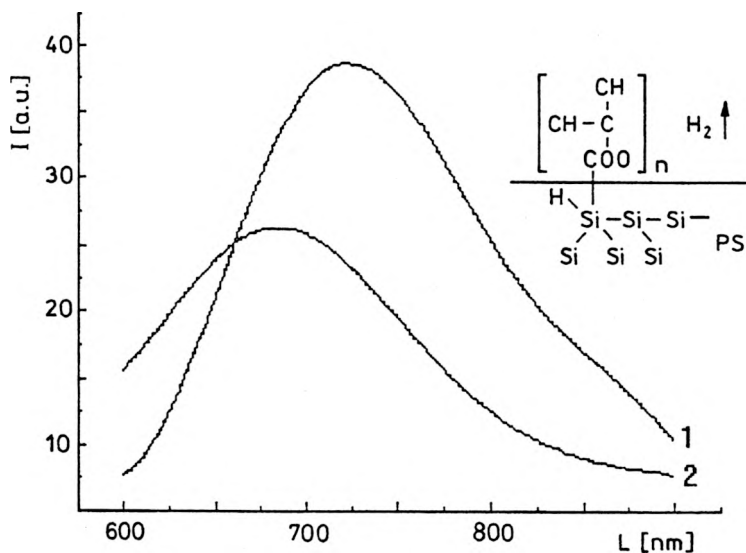
Fig. 1. Photoluminescence spectra of PS without thin film coating (1) and with polymer film coating (2). Insertion: the model of polymer (PMA) adsorption on PS surface.
