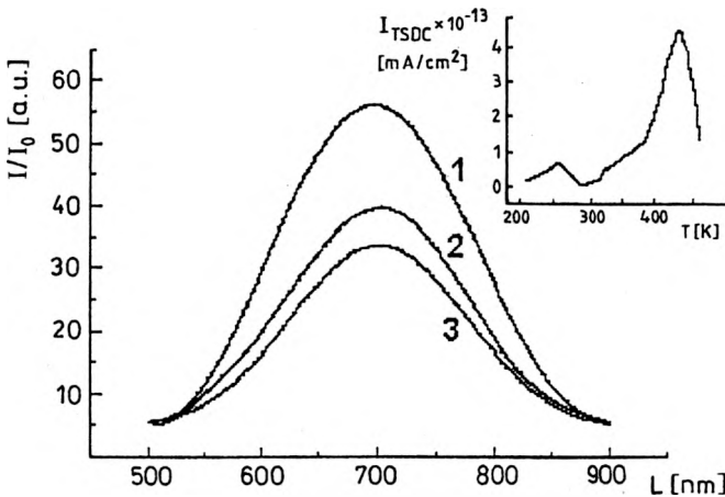
Fig. 3. The EL spectrum of PS in electrolyte: 1 – initial time moment, 2 – after 5 min, 3 – after 10 min. Insertion: the TSDC spectra of PS-Si heterostructure.
