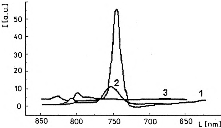
Fig. 2. Photoluminescence spectra of \text{SiO}_2 -PS (1), \text{Al}_2\text{O}_3 -PS (2), \text{ZnS} -PS (3) heterostructures.
