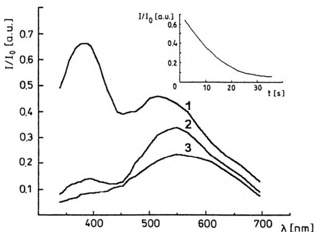
Fig. 4. CL PS spectrum at 77 K (1, 2) and 300 K (3) at initial time moment (1, 3) and after 20 min. (2). Insertion: CL intensity decreasing at \lambda_{\max}
