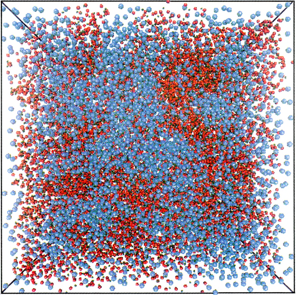
Fig. 3. Snapshot of atom configuration in the last simulation step for 0.5 Bi 0.5 SiO 2 system. Red balls – oxygen atoms, green balls – silicon atoms, bluish balls – bismuth atoms. 20000 atoms in the simulation box (6000 Bi atoms, 5000 Si atoms, 10 000 O atoms).
