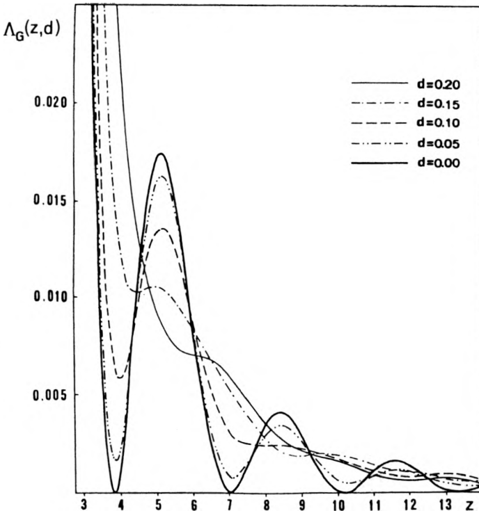
Fig. 5. Decay of the diffraction rings for the quasi-monodisperse medium of Gauss distribution \rho_G(D) with the increase of the relative standard deviation d .
