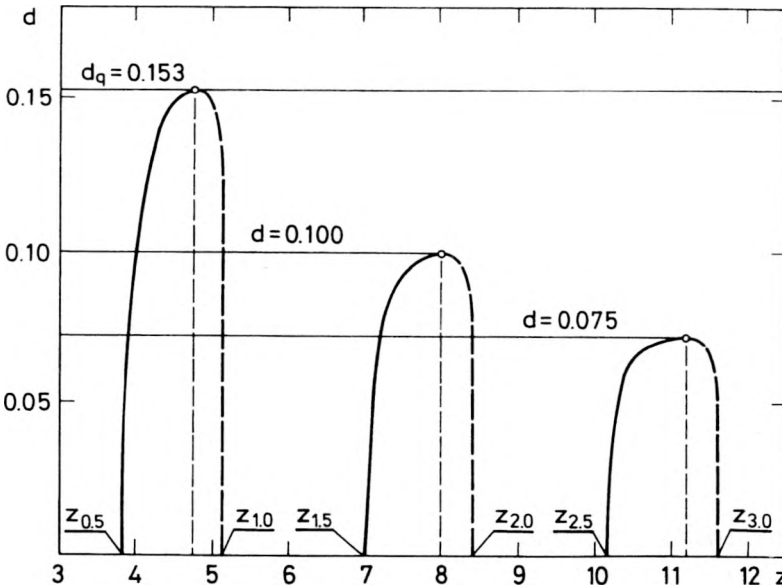
Fig. 7. Change of position of six consecutive extrema of light intensity \Lambda_G(z, d) for a quasi-monodisperse medium of Gauss distribution \rho_G(D) .
