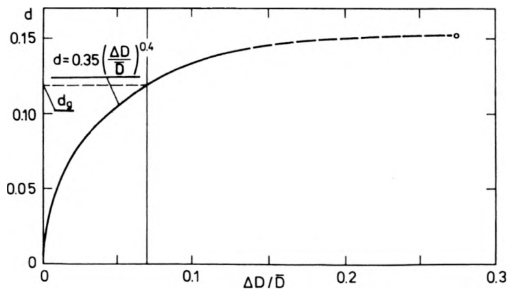
Fig. 12. Mutual dependence between the relative standard deviation d and the relative difference of diameters \Delta D/\bar{D} .
