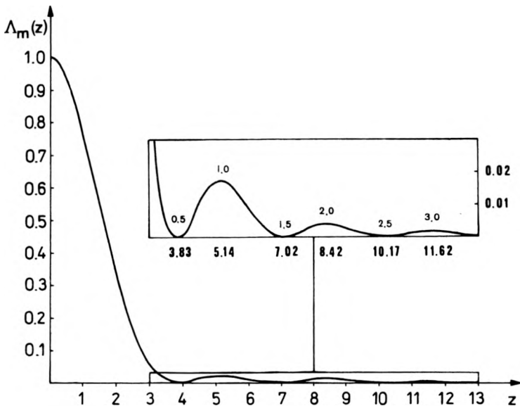
Fig. 4. Dimensionless intensity distribution of the light diffracted on a single drop.
