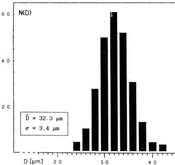
Fig. 14. Histogram of the drop pulverization spectrum of the starting injector of K 108-767 type of the Lis-5 engine produced by the photographic method.
