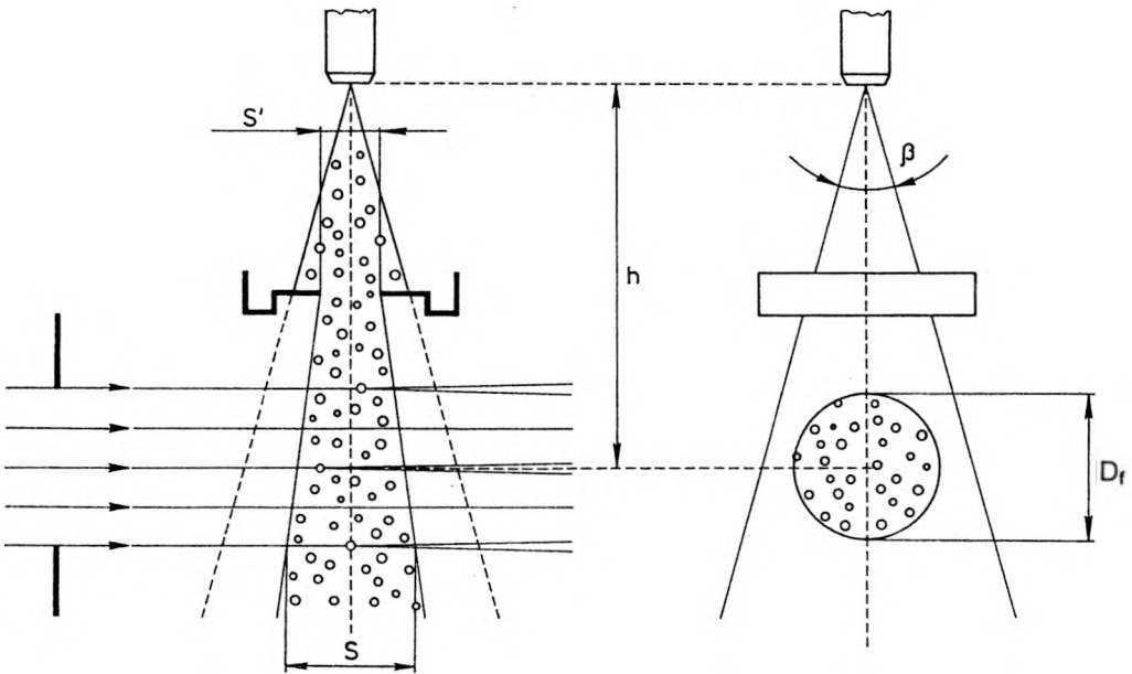
Fig. 1. Reduction of the measurement space by mechanical restriction of pulverization cone.
