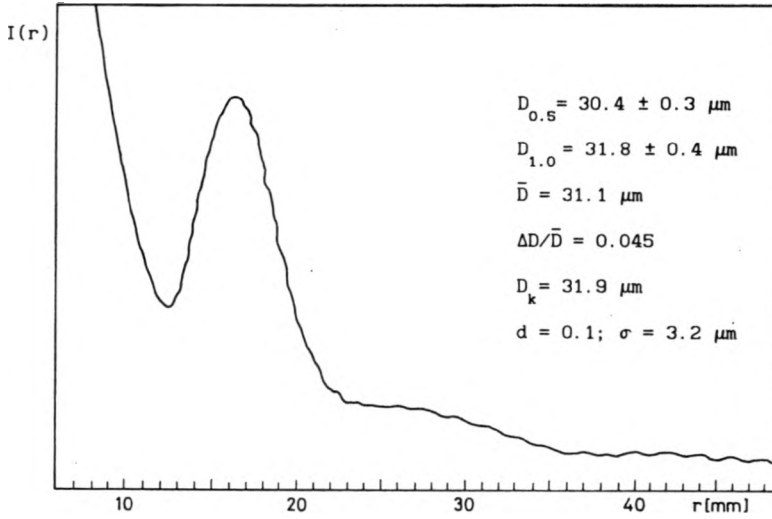
Fig. 13. Light intensity distribution I(r)/I(0) after the light wave passed through the pulverisation cone of the starting injector of K 108-767 type of the Lis-5 engine (pressure of the fuel forcing p = 0.5 MPa, the fuel delivery Q(p) = 8 l/h, angle of the pulverization cone \beta = 70^\circ , h = 250 mm, D_f = 50 mm, s = 2 mm, f = 0.5 m).
