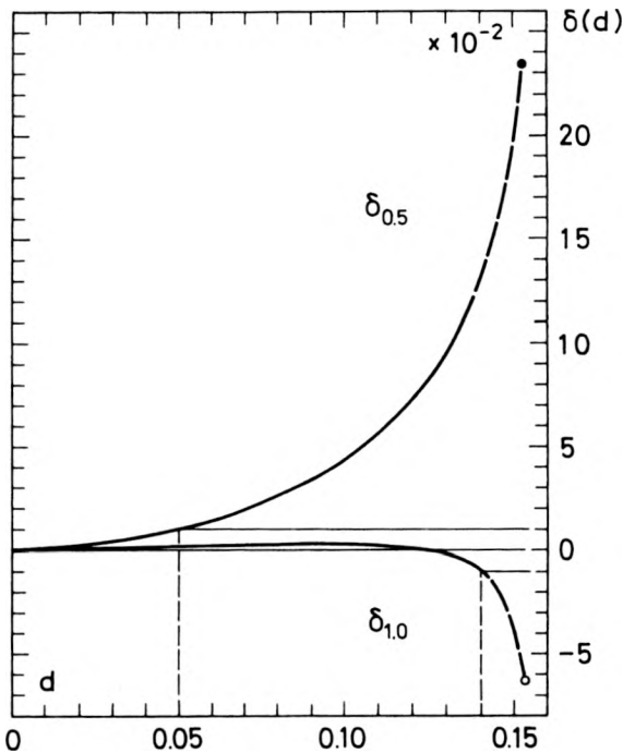
Fig. 9. Relative error \delta(d) of the position z_i(d) of the light intensity extrema.
