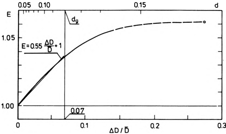
Fig. 10. Dependence of the correcting coefficient E on the relative difference \Delta D/\bar{D} .
