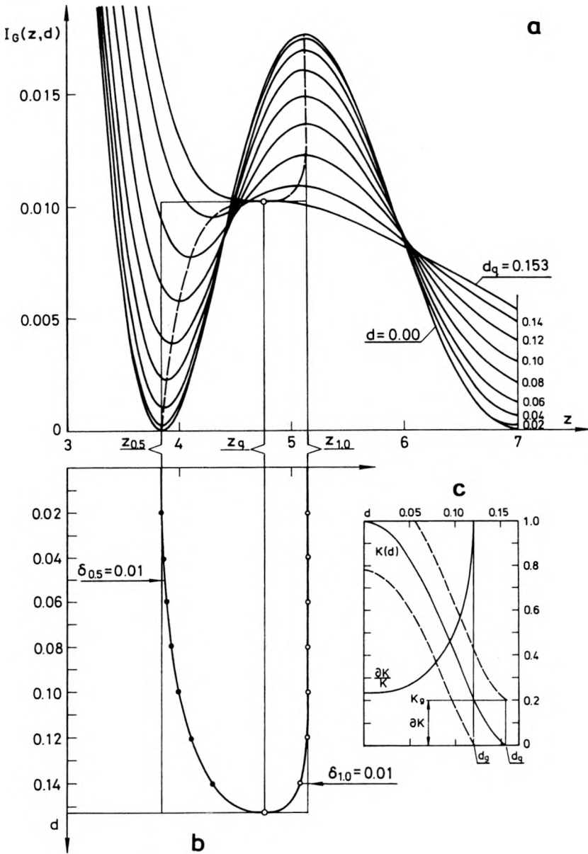
Fig. 6. Decay of the first dark and bright diffraction rings for a medium of normal distribution \rho_G(D) (a). The change of position of the light intensity extrema z_{0.5} and z_{1.0} versus the relative standard deviation d (b). Contrast K(d) between bright and dark diffractive rings (c).
