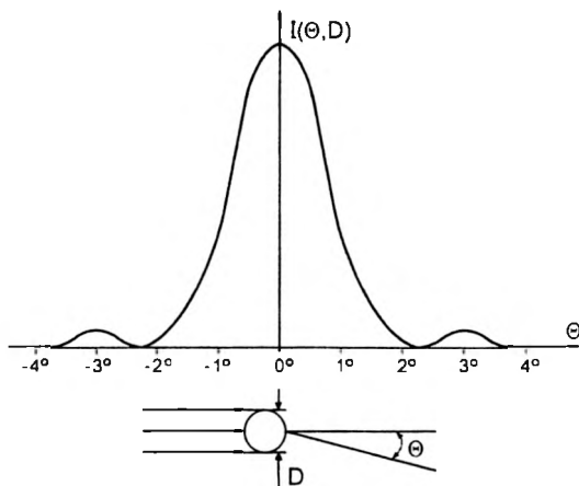
Fig. 2. Intensity distribution I(\theta, D) of the light scattered by a drop of diameter D = 20 \mu\text{m} illuminated by a plane wave of wavelength \lambda = 0.63 \mu\text{m} depending on the observation angle \theta .
