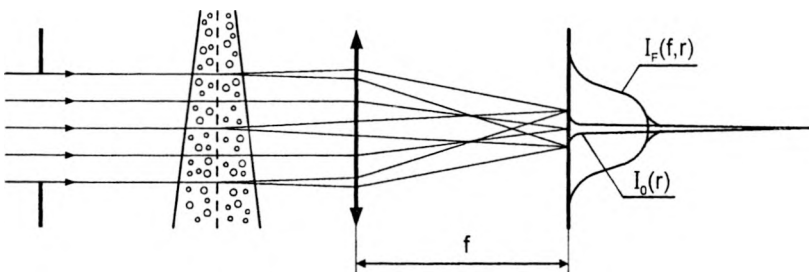
Fig. 3. Intensity distribution of the light in the focal plane after a plane wave passed through the aerosol stream.
