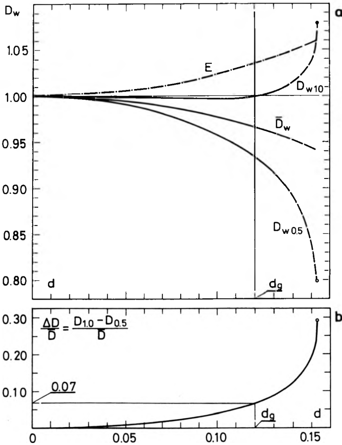
Fig. 8. Dependence of dimensionless diameters D_{w0.5} , D_{w1.0} , \bar{D}_w of relative difference \Delta D/\bar{D} and the correcting coefficient E on the parameter d = \sigma/D .
