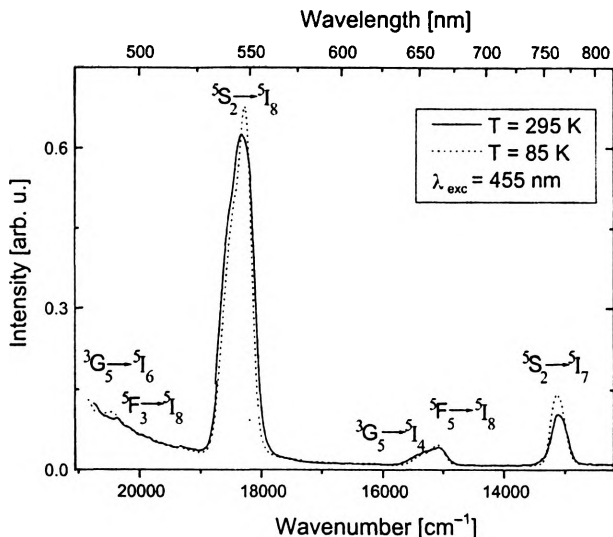
Fig. 2. Photoluminescence spectra of the Ho-doped glasses with 3\text{CaO-Ga}_2\text{O}_3-3\text{GeO}_2 composition, registered at T = 295\text{ K} and T = 85\text{ K} .
