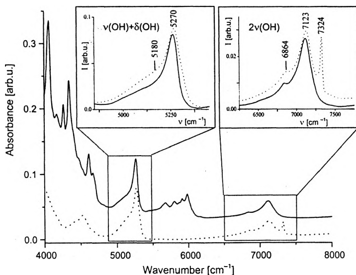
Fig. 1. NIR absorption spectra of PG (type II) with pore diameter 4 nm (PG4) (dashed line) and nanocomposite system PG + 5CB (solid line). The inserts show fragments of the spectra in the regions of the first overtone 2\nu(\text{OH}) and combination tone \nu(\text{OH}) + \delta(\text{OH}) of OH stretching and bending vibrations of adsorbed water molecules and Si-OH groups.
