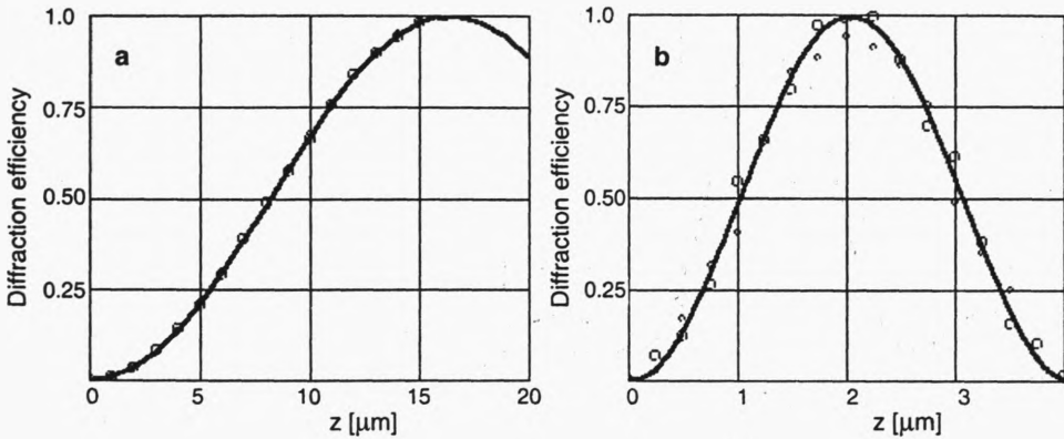
Fig. 2. Plot of diffraction efficiency \eta_1(z) for \tilde{\epsilon} \approx 0.0505 (a) and \tilde{\epsilon} \approx 0.404 (b).
