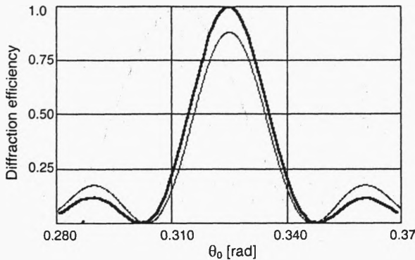
Fig. 3. Relationship between the diffraction efficiency and the angle \theta_0 for TM-polarization (thick line) and for TE-polarization (thin line).
