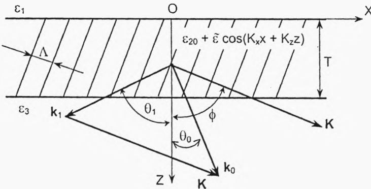
Fig. 1. Schematic representation of incident and diffracted plane waves and a periodic volume grating ( T is the thickness of grating in the direction of axis OZ ).
