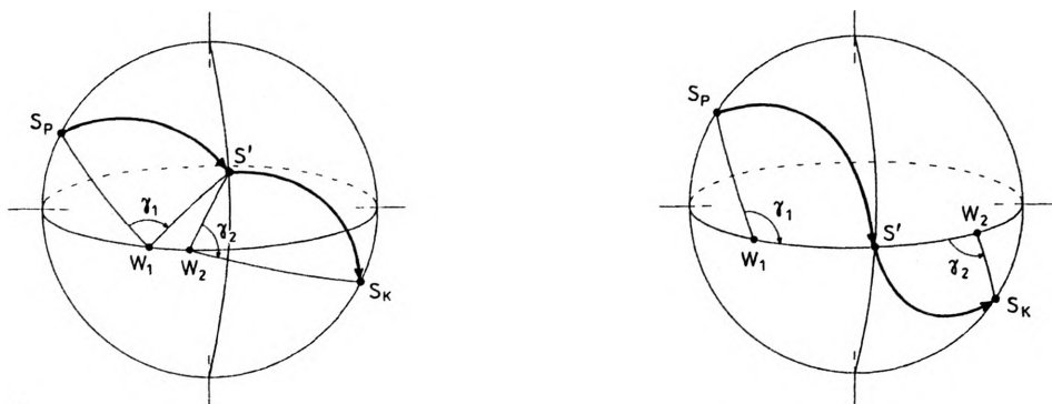
▲ Fig. 4. Transformation of the polarization state of light into the orthogonal one.
