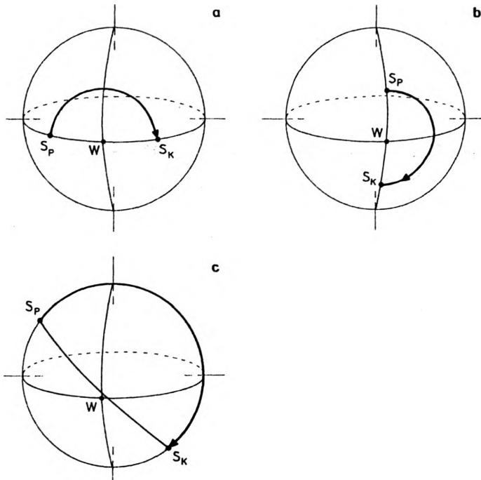
Fig. 1. Three most important cases of using the half-wave plates in optical setups: change of the azimuth angle of linearly polarized light (a); change of the sign of the ellipticity of light (b); change of the polarization state of light into perpendicular one (c).
