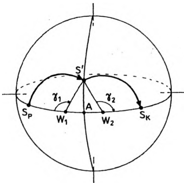
Fig. 2. Transformation of the azimuth angle of linearly polarized light.
