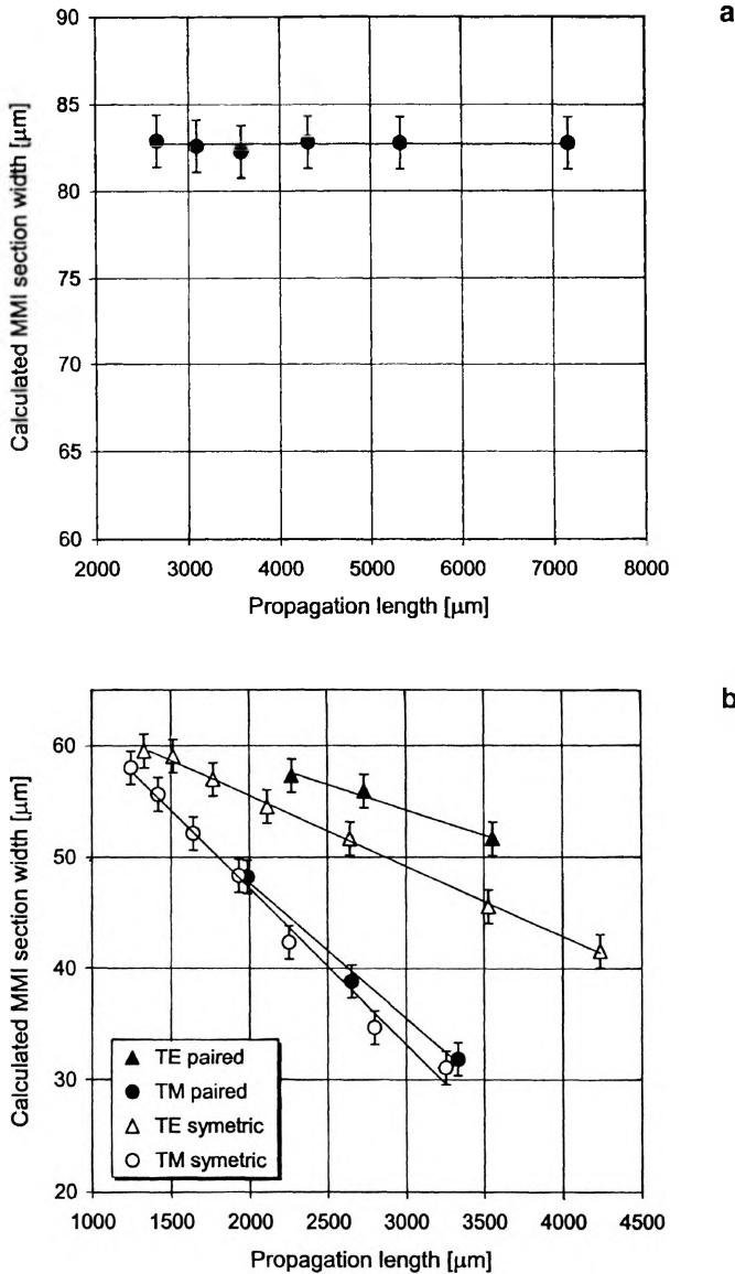
Fig. 11. Dependence of calculated MMI section width on the propagation length; a – MMI section of the width 81 μm, made by \text{Ag}^+\text{-Na}^+ ion exchange, b – MMI section of the width 60 μm, made by \text{K}^+\text{-Na}^+ ion exchange.
