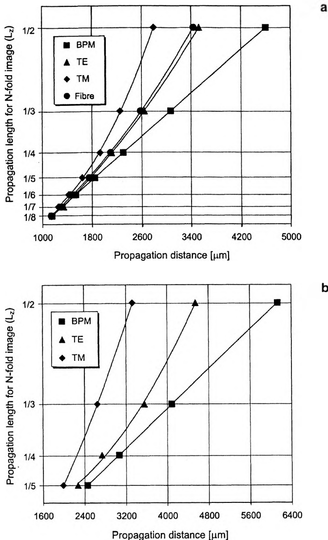
Fig. 10. Comparison between experimental and theoretical dependences of lengths of N -fold images on propagation length; MMI section of the width 60 \mu\text{m} , made by \text{K}^+\text{-Na}^+ ion exchange; a – symmetric interference, b – paired interference.
