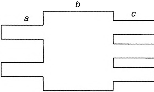
Fig. 1. Scheme of MMI structure: group of single-mode waveguides ( a ), multimode section ( b ), single-mode output waveguides ( c ).
