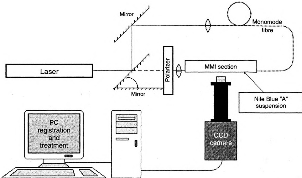
Fig. 3. Experimental arrangement, from [5].
