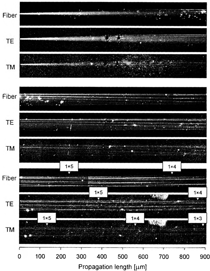
Fig. 7. Successive sequences of recorded mode field interference images for MMI section of the width 60\ \mu\text{m} , made by \text{K}^+\text{-Na}^+ ion exchange, excited at one third of the section width.
