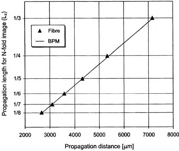
Fig. 8. Comparison between experimental and theoretical dependences of propagation lengths for N -fold images on the propagation distance; MMI section of the width 81 \mu\text{m} , made by \text{Ag}^+\text{-Na}^+ ion exchange, excited at one third of the section width.
