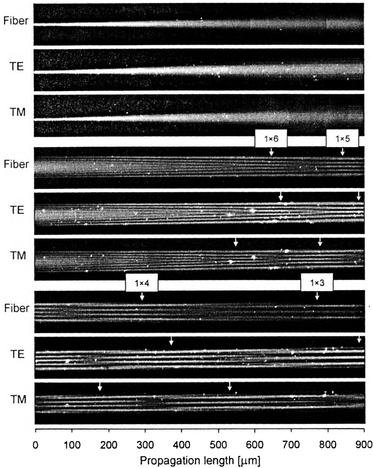
Fig. 6. Successive sequences of recorded mode field interference images for MMI section of the width 60\ \mu\text{m} , made by \text{K}^+\text{-Na}^+ ion exchange, symmetrically excited.
