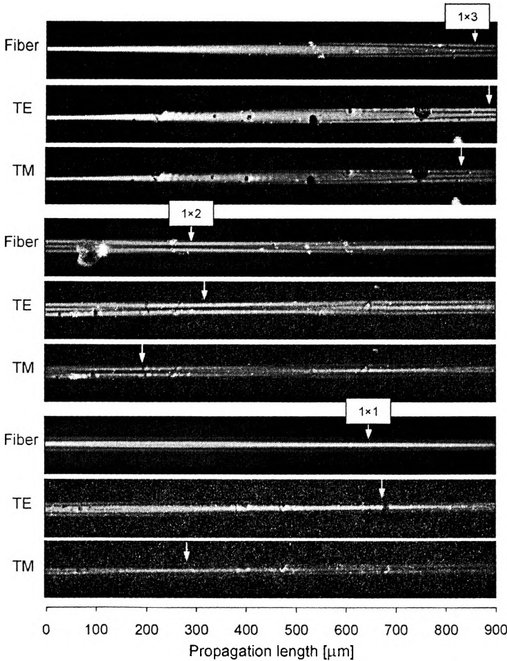
Fig. 5. Successive sequences of recorded mode field interference images for MMI section of the width 30 \mu\text{m} , made by K^+Na^+ ion exchange, symmetrically excited.
