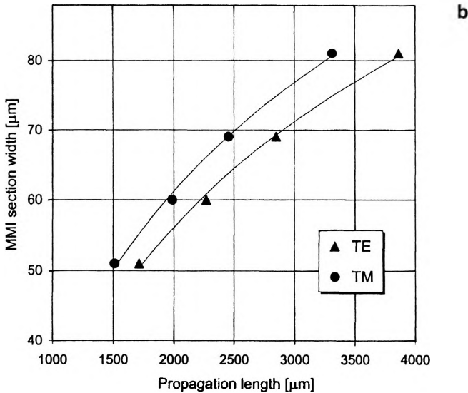
Fig. 9. Dependence of length of N -fold images on the window width for MMI section made by \text{K}^+ - \text{Na}^+ ion exchange; a – for symmetric interference, b – for paired interference.
