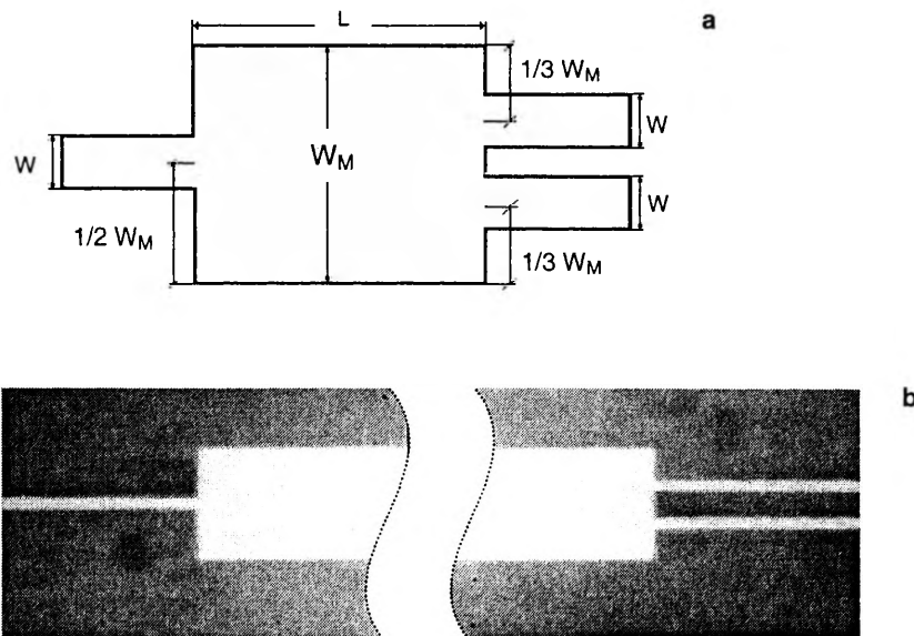
Fig. 2. Geometry of the mask designed (a) and micro-image of the end of the mask (b).
