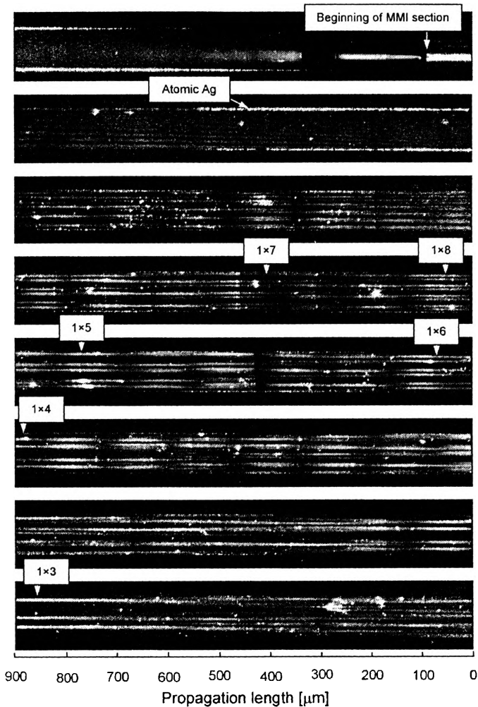
Fig. 4. Successive sequences of recorded mode field interference images for MMI section of the width 81\ \mu\text{m} , made by \text{Ag}^+ - \text{Na}^+ ion exchange, excited at one third of the section width.
