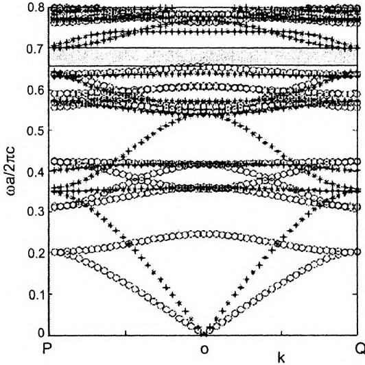
Fig. 2. Photonic band structures for E (denotes as ○) and H (denotes as *) polarizations of 2D square compound lattice.
