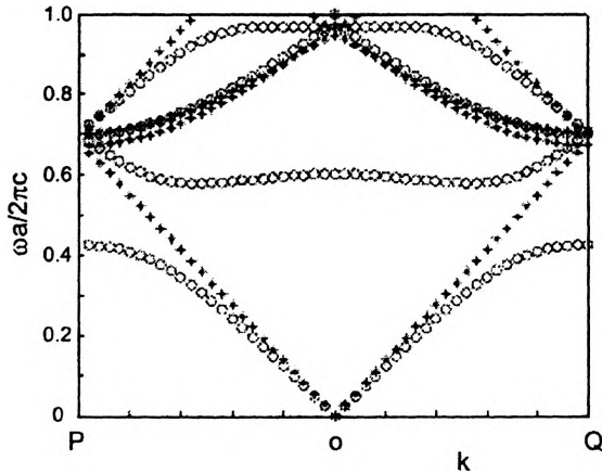
Fig. 3. Photonic band structures for E (denotes as \circ ) and H (denotes as * ) polarizations of 2D square single lattice.
