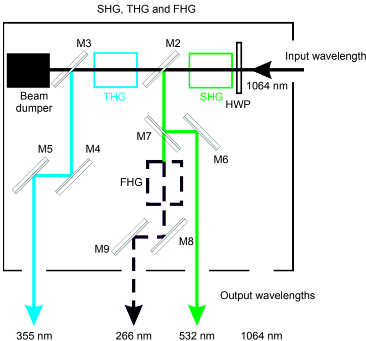
Fig. 5. An optical scheme of a laser frequency conversion system.
