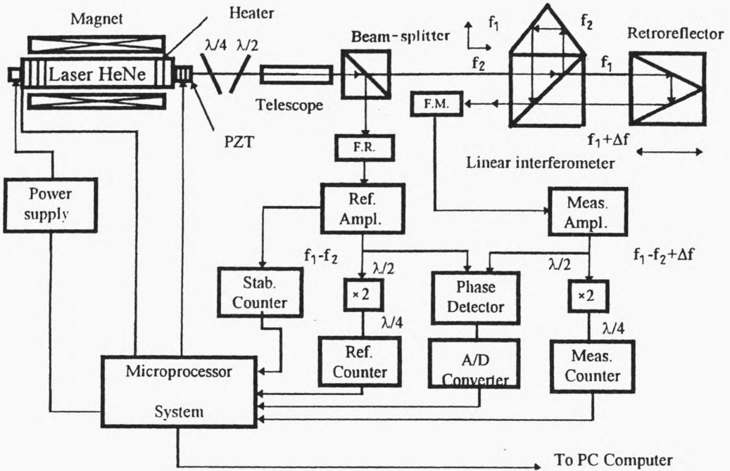
Fig. 2. Block diagram of laser head. \lambda/4 – quarter-wave plate, \lambda/2 – half-wave plate, F.M. – measurement photodetector, F.R. – reference photodetector, \times 2 – multiplier by 2, PZT – piezoceramic
