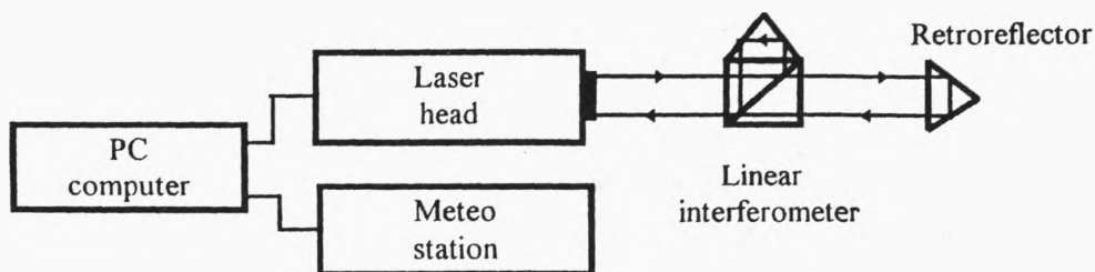
Fig. 1. Block diagram of the laser interferometer LSP-30
