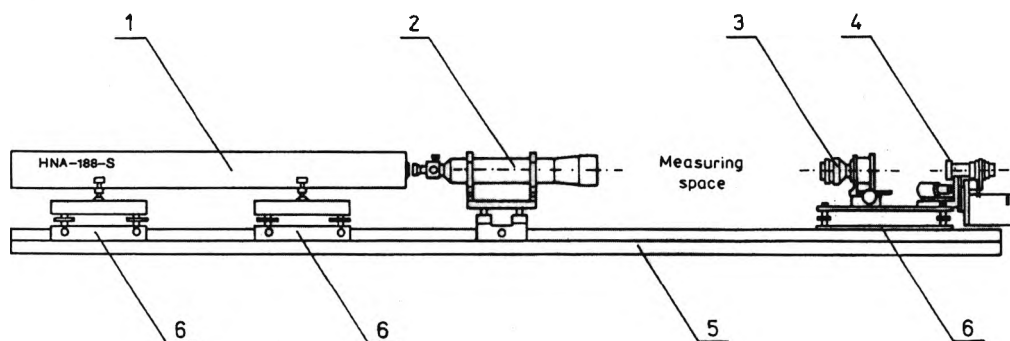
Fig. 6. Measuring stand for recording the diffraction images (1 — gas HNA-188-S laser, 2 — ZHL-UO telescope, 3 — Fourier transforming objective, 4 — scanning and light intensity measuring system, 5 — optical bench, 6 — adjustment stage).
