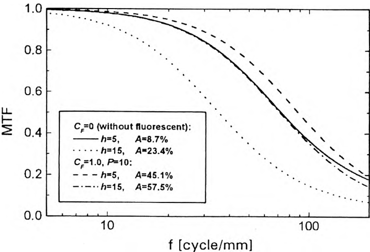
Fig. 3. The MTF curves for the layers of 5 and 15 \mu\text{m} in thickness, without fluorescent substance and for relative concentration of the fluorescent substance C_F = 1.0 and the parameter P = 10 . In the legend the calculated values of the effective light absorption A are given.
