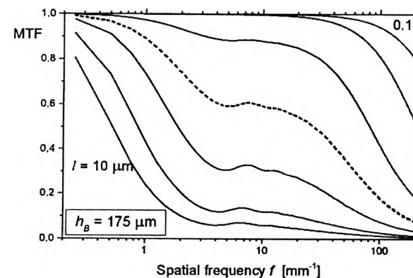
Fig. 7. MTF of the light-sensitive system for the case of variable average free path of the photon l = 0.1, 0.2, 0.5, 1, 2, 5 and 10 \mu\text{m} , for the base thickness h_B = 175 \mu\text{m} .
