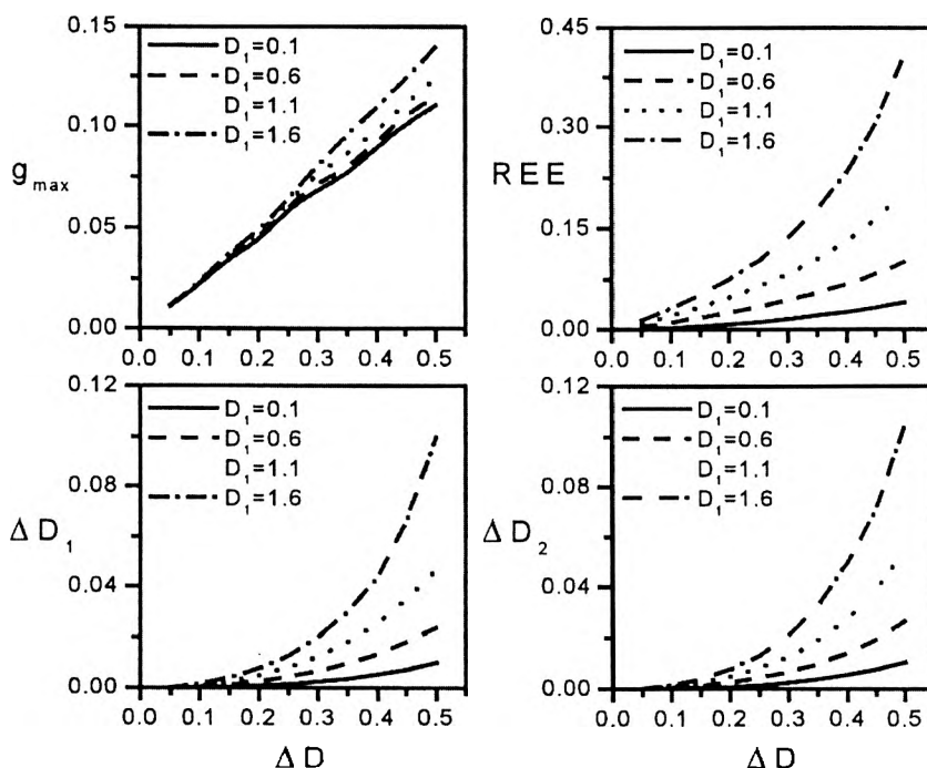
Fig. 4. Changes in maximal gradient of the limiting curve ( g_{\max} ) and the intensity of edge effects action expressed in terms of REE indicator and the optical density differences \Delta D_1 and \Delta D_2 determined as a function of optical density difference in the image and the background ( \Delta D ). These values were obtained for four levels of background optical density ( D_1 ) amounting to 0.1, 0.6, 1.1 and 1.6, respectively. The calculations were carried out for the irradiation-sensitive layer of contrast equal to unity.
