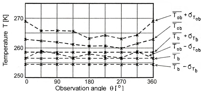
Fig. 5. Statistical measures of temperature distributions of an actual target and background as a function of the observation angle (thermovision measuring camera).
