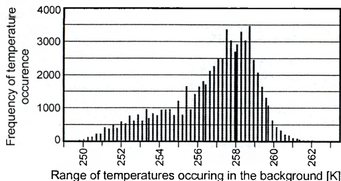
Fig. 2. Histogram of background temperature distribution for the observation angle of 180^\circ (thermovision measuring camera).
