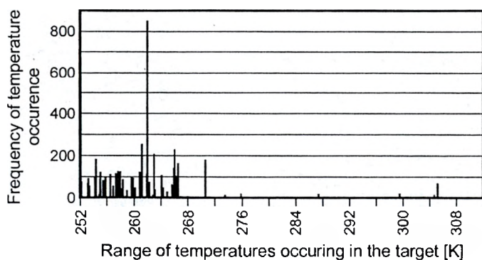
Fig. 3. Histogram of temperature distribution on target surface for the observation angle of 180^\circ (FTTM).
