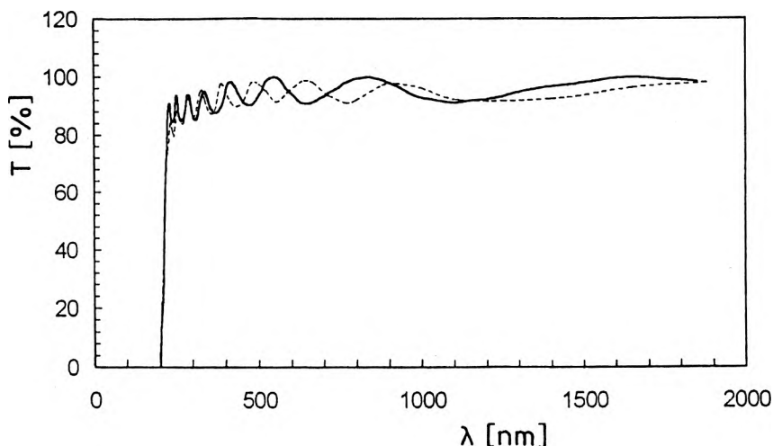
Fig. 1. Spectral dependence of the transmission coefficient T(\lambda) of lutetium oxide thin films deposited under different evaporation conditions. The broken line shows the T(\lambda) curve for films deposited at the oxygen pressure of 8 \times 10^{-5} Tr ( 1 \times 10^{-2} Pa) and at the substrate temperature of 423 K. Film thickness d = 513 nm. The solid line shows the T(\lambda) curve for films deposited at the residual gas pressure of 5 \times 10^{-6} Tr ( 7 \times 10^{-4} Pa) and at the substrate temperature of 423 K. Film thickness d = 457 nm.
