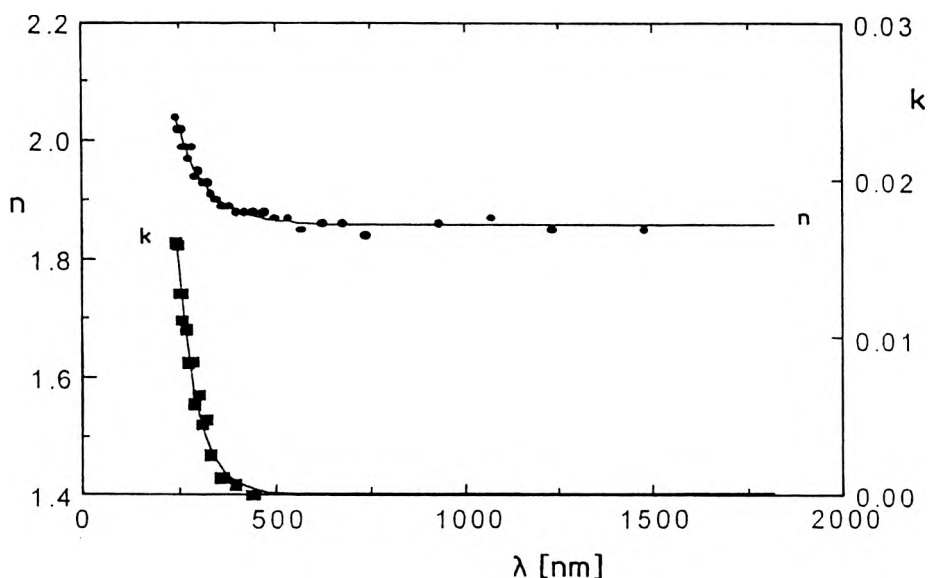
Fig. 3. Spectral dependence of the refractive index n and extinction coefficient k for \text{Lu}_2\text{O}_3 thin films deposited onto quartz substrate. Sample thickness – 997 nm.
