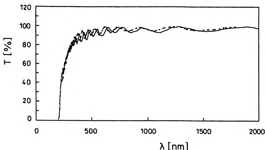
Fig. 2. Spectral dependence of the transmission coefficient T(\lambda) for as-deposited oxide thin films (solid line) and for films annealed at a temperature of 523 K for 24 h (dotted line). Sample thickness – 997 nm.
