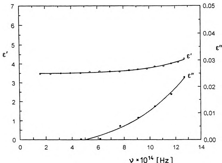
Fig. 5. Frequency dependence of the real part \epsilon' and imaginary part \epsilon'' of the complex dielectric function \epsilon^*(\nu) for \text{Lu}_2\text{O}_3 thin films.
