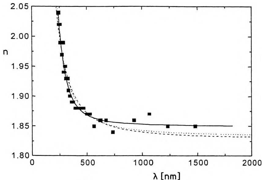
Fig. 4. Spectral dependence of the refractive index for \text{Lu}_2\text{O}_3 thin films of a thickness of 997 nm – comparison between the experimental data and the data calculated from Eqs. (1)–(3). The dotted line shows the best fit from Eq. (1). The solid line presents the best fit according to Eq. (2). The dashed line shows the best fit from Eq. (3).
