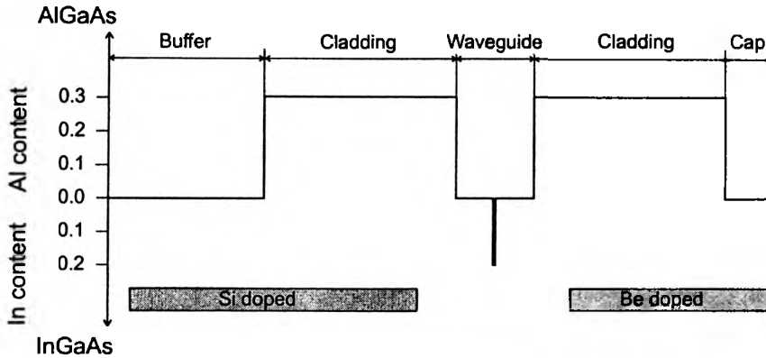
Fig. 1. InGaAs/GaAs quantum-well laser structure.
