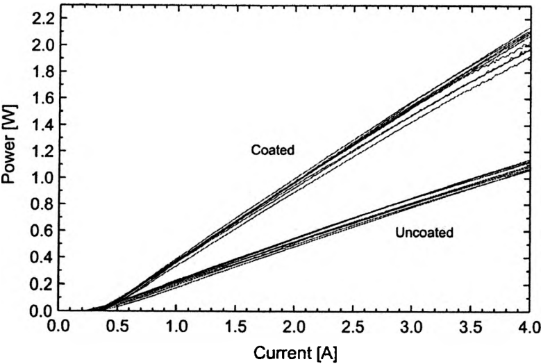
Fig. 4. Typical pulsed light-current characteristics of the InGaAs/GaAs lasers.
