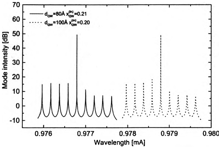
Fig. 3. Calculated spectral characteristics of the InGaAs/GaAs lasers with different combination of the thickness and indium content of the QW layer: d_{\text{QW}} = 80 \text{ \AA} and x_{\text{QW}}^{(\text{In})} = 0.21 (solid line), d_{\text{QW}} = 100 \text{ \AA} and x_{\text{QW}}^{(\text{In})} = 0.20 (dashed line). The waveguide layer thickness d_w = 0.3 \text{ \mu m} .
