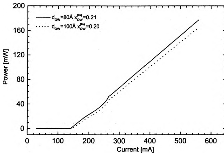
Fig. 2. Calculated light-current characteristics of the InGaAs/GaAs lasers with different combination of the thickness and indium content of the QW layer: d_{\text{QW}} = 80 \text{ Å} and x_{\text{QW}}^{(\text{In})} = 0.21 (solid line), d_{\text{QW}} = 100 \text{ Å} and x_{\text{QW}}^{(\text{In})} = 0.20 (dashed line). The waveguide layer thickness d_w = 0.3 \mu\text{m} .
