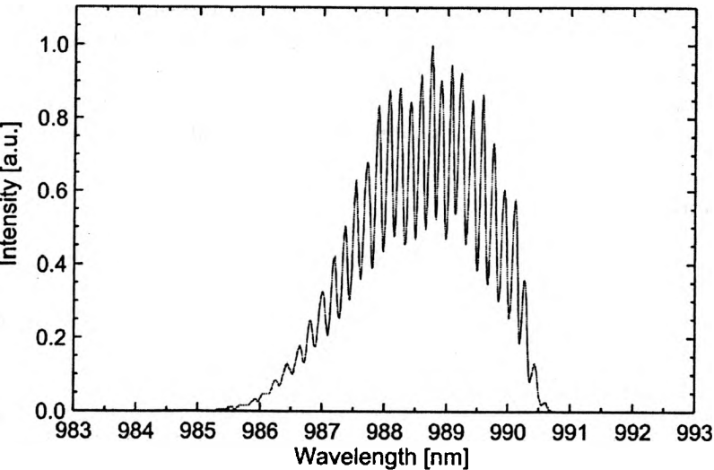
Fig. 5. Typical emission spectrum of the InGaAs/GaAs laser.
