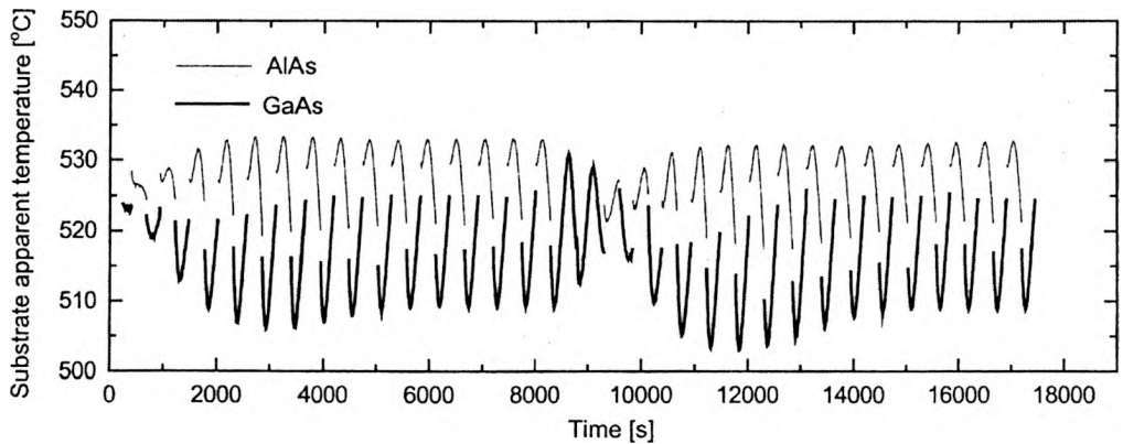
Fig. 2. Pyrometer readout during the MBE growth of \text{In}_{0.2}\text{Ga}_{0.8}\text{As}/\text{GaAs} VCSEL structure.
