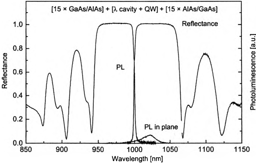
Fig. 5. Reflectance, photoluminescence perpendicular to the Bragg reflector, and photoluminescence from the edge of the structure (PL in plane) of \lambda -sized \text{In}_{0.2}\text{Ga}_{0.8}\text{As}/\text{GaAs} planar microcavity, resonant at 1000 nm.
