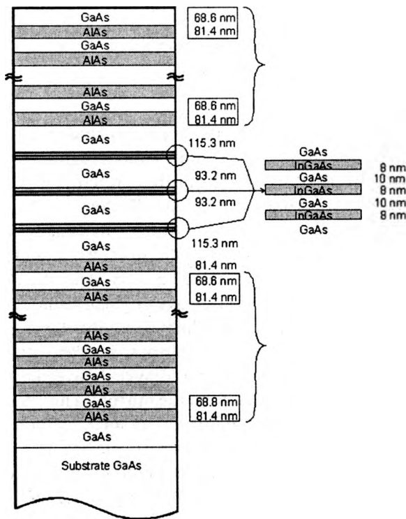
Fig. 7. Schematic VCSEL structure with 3\times 3 InGaAs QW active region designed for operation at 1\text{ }\mu\text{m} at T = 300\text{ K} .
