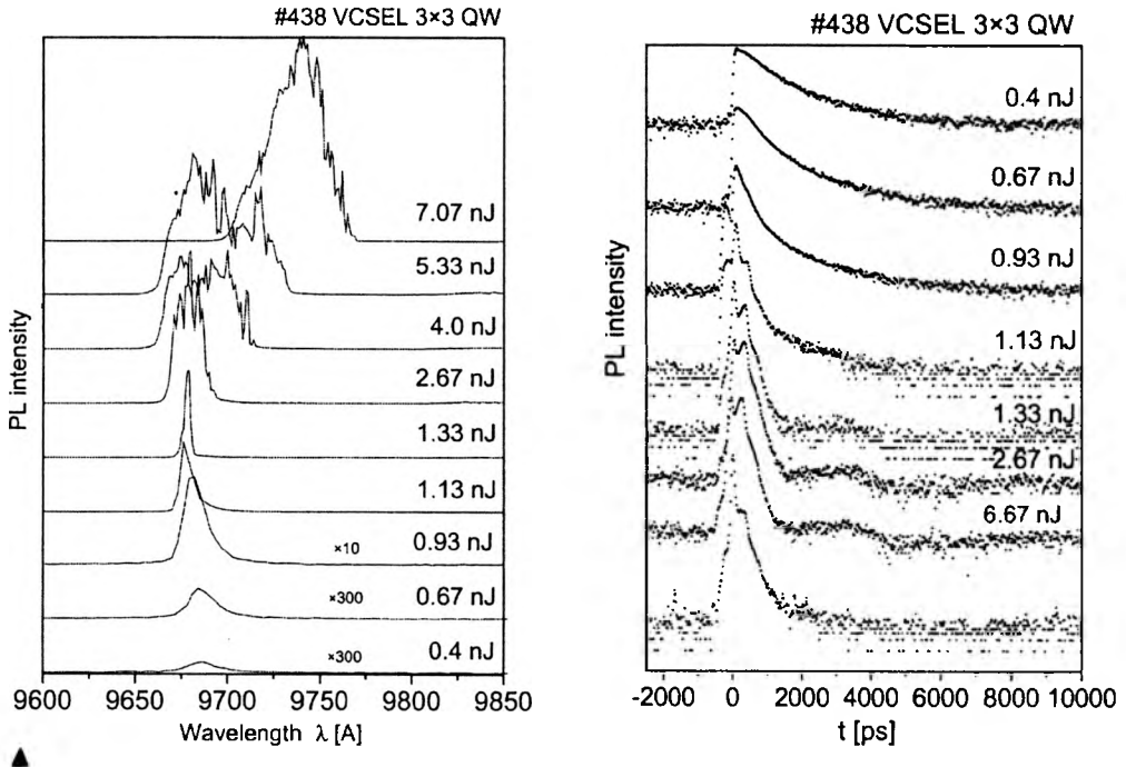
Fig. 8. Emission spectra of 3x3 QW InGaAs VCSEL structure under optical pumping.
