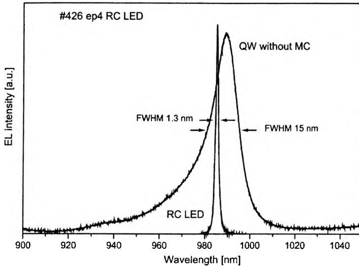
Fig. 13. Emission spectrum of RC LED compared to conventional LED.
