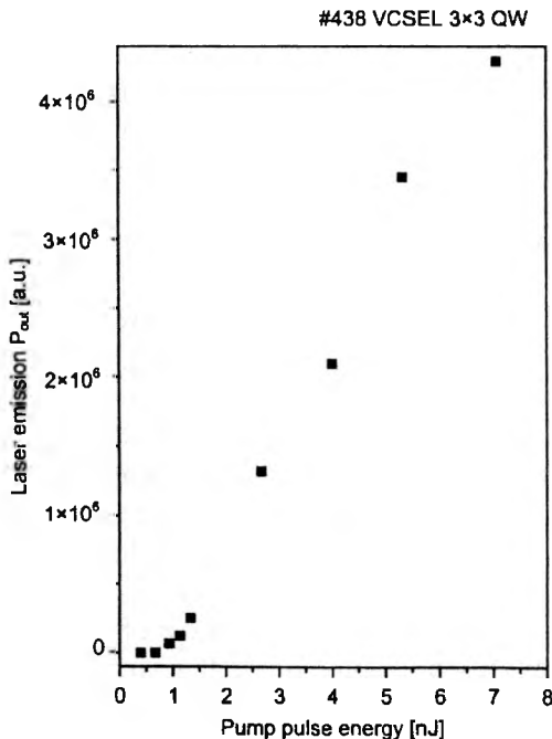
Fig. 10. Emission intensity vs. pumping pulse energy for 3 \times 3 QW InGaAs VCSEL structure.
