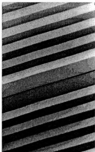
Fig. 3. TEM pictures of \lambda -sized \text{In}_{0.2}\text{Ga}_{0.8}\text{As}/\text{GaAs} planar microcavity. The structure has been grown by MBE at the Department of Physics and Technology of Low Dimensional Structures of the Institute of Electron Technology. The bright regions in the photograph refer to AlAs, the dark region refer to GaAs; the narrow dark line in the middle of the cavity refers to InGaAs QW.
