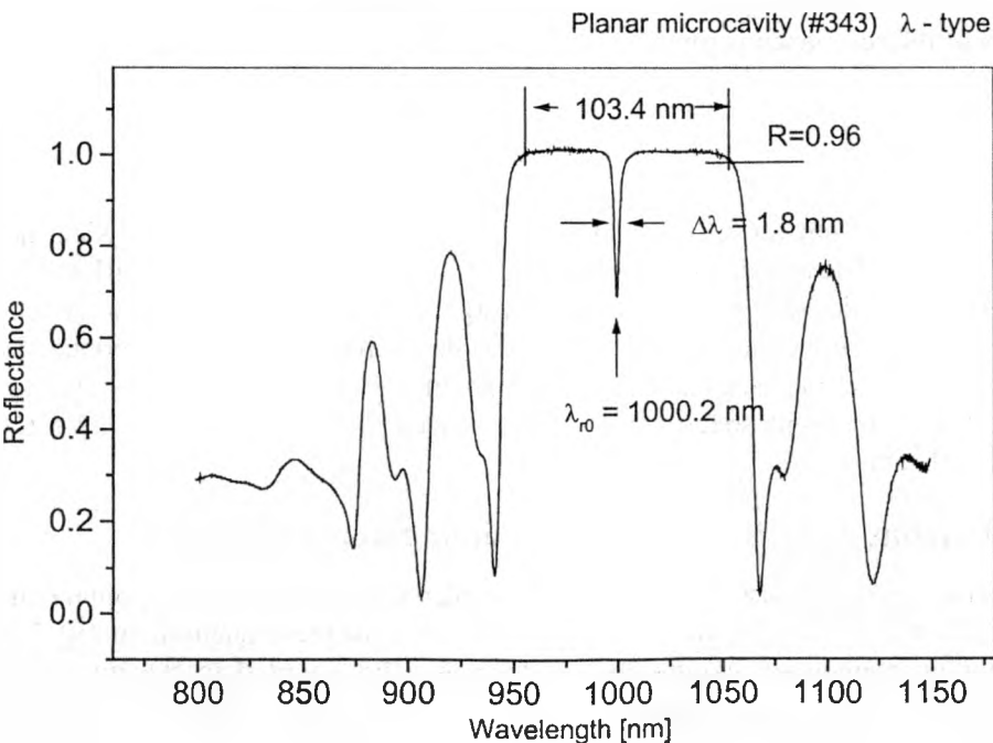
Fig. 4. Refeactance spectrum of \lambda -sized \text{In}_{0.2}\text{Ga}_{0.8}\text{As}/\text{GaAs} planar microcavity, resonant at 1000 nm.
