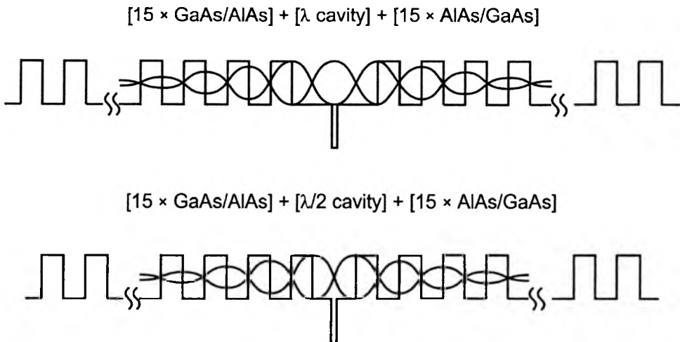
Fig. 1. Schematic illustration of the band diagram of the \lambda -sized and \lambda/2 -sized microcavities. Note the shape of the standing wave pattern in both cases.
