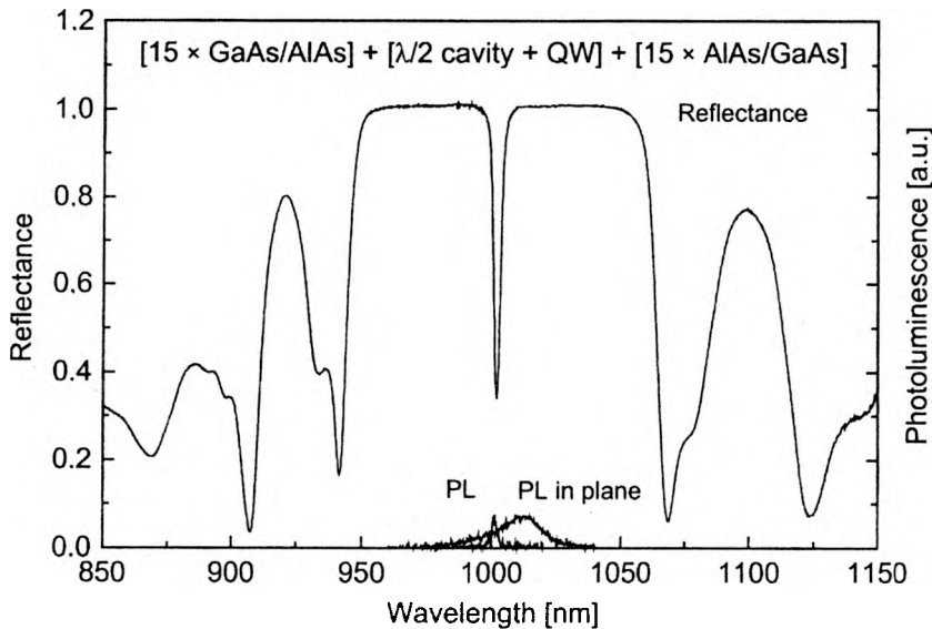
Fig. 6. Reflectance, photoluminescence perpendicular to the Bragg reflector and photoluminescence from the edge of the structure (PL in plane) of \lambda/2 -sized \text{In}_{0.2}\text{Ga}_{0.8}\text{As/GaAs} planar microcavity, resonant at 1000 nm.
