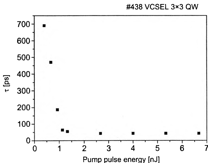
Fig. 11. Carrier lifetime vs. pumping pulse energy for 3×3 QW InGaAs VCSEL structure.
