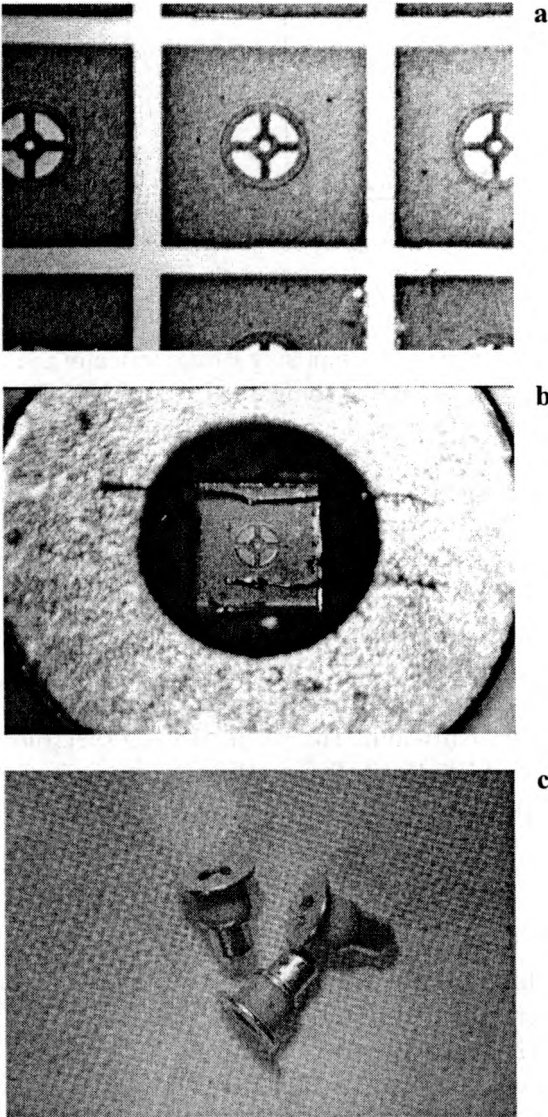
Fig. 12. RC LED structures on a wafer, before separating them into individual chips (a), view of the chip mounted inside the case (b), assembled diodes (c).
