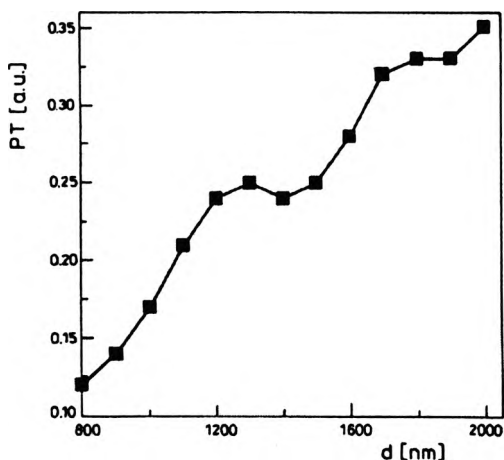
Fig. 2. Dependence of the maximal reversible PT as a function of film thickness for the wavelength 10.6 \mu\text{m} for the CO laser ( \lambda = 5.5 \mu\text{m} ) photoinduced photon fluxes about the 18 \times 10^{13} photon/cm 2 per pulse after 30 min of illumination.
