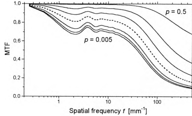
▲ Fig. 6. The MTF of the light-sensitive system with AH layer for variable photon absorption probability, p = 0.005, 0.01, 0.02, 0.05, 0.1, 0.2 and 0.5 . Fig. 7. The MTF of the light-sensitive system without AH layer for variable photon absorption probability, p = 0.005, 0.01, 0.02, 0.05, 0.1, 0.2 and 0.5 .
