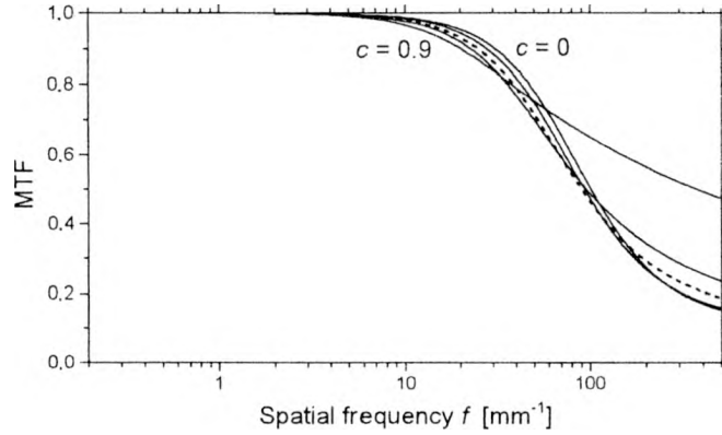
▲ Fig. 10. The MTF of the light-sensitive system with AH layer for variable elongation of elementary scattering indicatrix c = 0, 0.3, 0.55, 0.7 and 0.9 . Fig. 11. The MTF of the light-sensitive system without AH layer for variable elongation of elementary scattering indicatrix c = 0, 0.3, 0.55, 0.7 and 0.9 .
