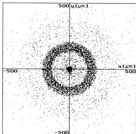
Fig. 2. Distribution of the light absorbed in the heterogeneous layer obtained in one of the computer simulations as a result of point irradiation of the model light-sensitive system. Black dots represent places in which photon absorption by the silver halide crystal occurred.
