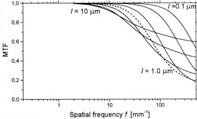
Fig. 8. The MTF of the light-sensitive system with AH layer for variable average free paths of the photon, l = 0.1, 0.2, 0.5, 1, 2, 5 and 10 \mu\text{m} . Fig. 9. The MTF of the light-sensitive system without AH layer for variable average free paths of the photon, l = 0.1, 0.2, 0.5, 1, 2, 5 and 10 \mu\text{m} .
