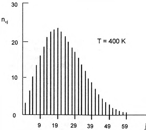
Fig. 2. Population n_{vj} of the rotational levels j of \text{CO}_2 molecule.
