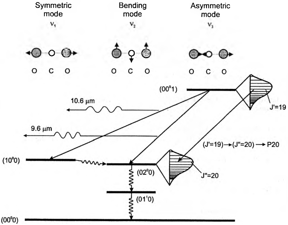
Fig. 1. Simplified system of energy levels of a \text{CO}_2 molecule ( \text{N}_2 molecule is not indicated).
