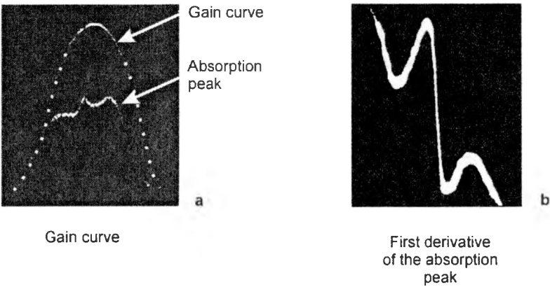
Fig. 32. CO 2 emission line with SF 6 absorption peak (a) and first derivative signal of the peak (b) – experimental data [35].
