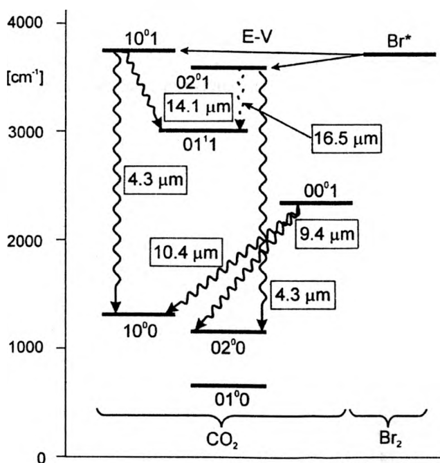
Fig. 23. Energy-level diagram of the \text{Br}^*\text{-CO}_2 system [13].
