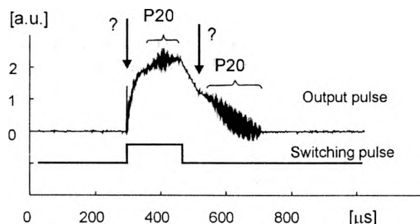
Fig. 8. Output laser pulse from the slab-waveguide CO 2 laser in pulse regime. Laser jumps from one emission line to another during the pulse duration [36].
