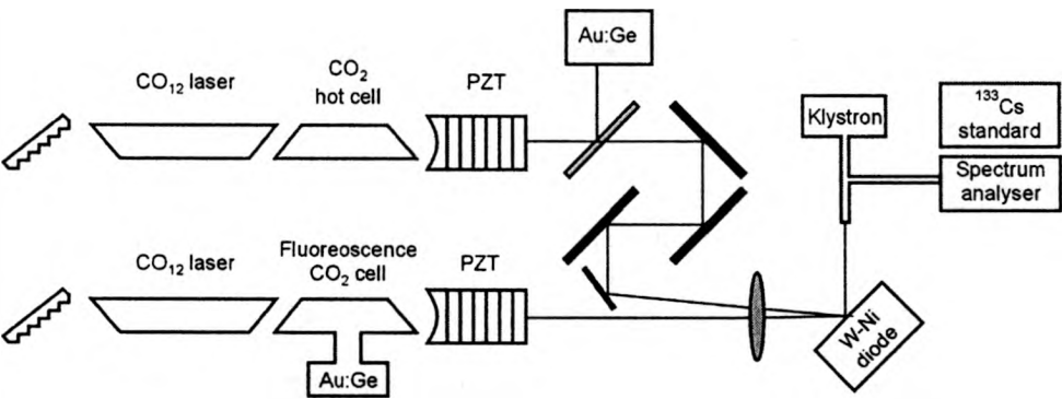
Fig. 5. Setup for measurements of the beat frequencies between the sequence \nu_s and regular \nu_r lines of the CO 2 laser. Explanation in the main text.
