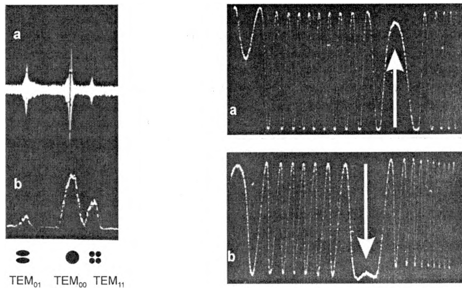
Fig. 6. Beat frequency signal obtained by heterodyning the single-mode \text{CO}_2 laser (a) and three-mode \text{CO}_2 laser [34] (b). Three modes are detected as a beat signal (a) and classical perturbations in the shape of the gain curve (b).
