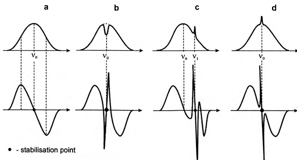
Fig. 31. Laser frequency stabilisation to the center of: a – emission line, b – Lamb dip, c – absorption peak, d – absorption peak in the centre of the line.
