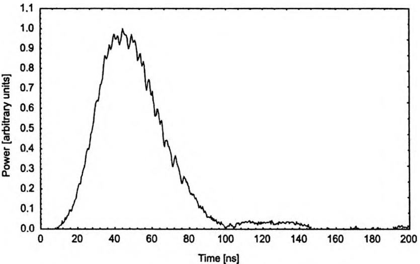
Fig. 8. Oscillogram of a laser giant pulse; pump energy E_p = 19.2 J, pulsewidth \tau_i = 37 ns, transmission of the output mirror T = 47\% .
