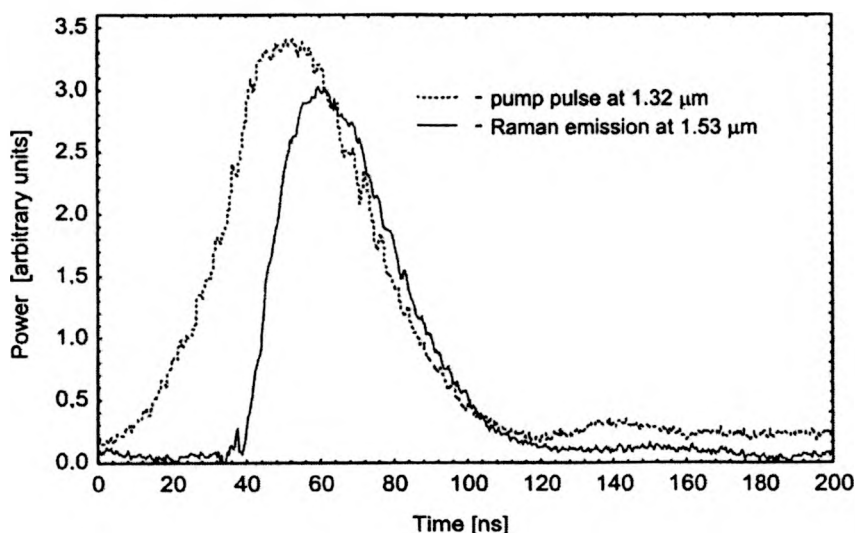
Fig. 10. Oscillogram of laser giant pulse at the line 1.318 \mu\text{m} and Raman emission at the wavelength 1.53 \mu\text{m} .
