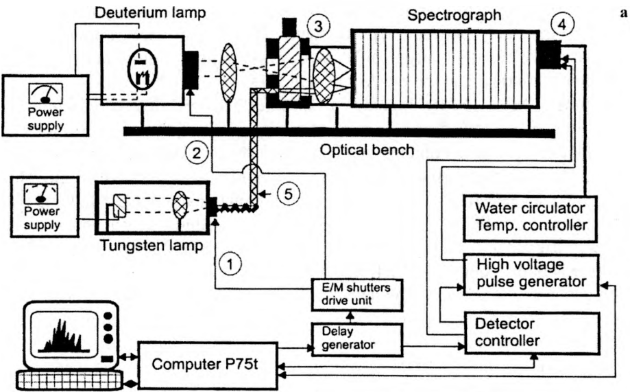
1, 2 – electromechanical shutters, 3 – sample cell holder, 4 – CCD optical detector, 5 – optical fiber
