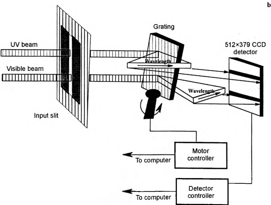
Fig. 1. Block diagram for the experimental setup (a). Optical paths of the UV and visible beams inside the spectrograph (b).
