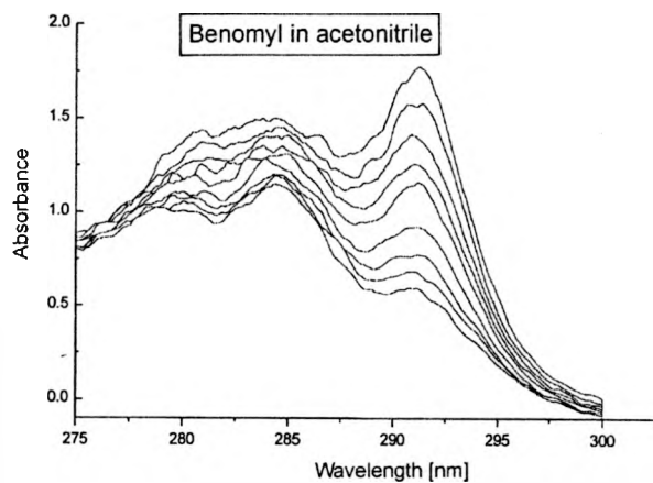
Fig. 4. The 2D UV spectra of 0.65 mg/L benomyl in \text{CH}_3\text{CN} for different periods of time.
