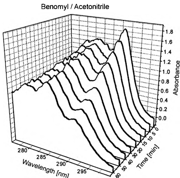
Fig. 5. The 3D UV spectra of 0.65 mg/L benomyl in \text{CH}_3\text{CN} and versus time (0–80 min).
