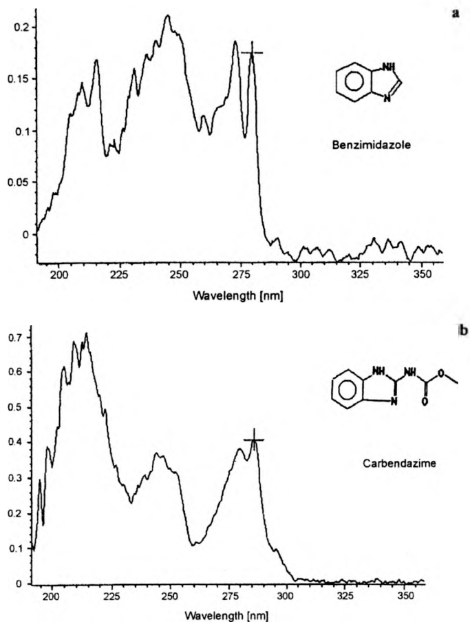
Fig. 3. The UV spectra of: 0.5 mg/L benzimidazole in \text{CH}_3\text{CN} (a) and 0.7 mg/L carbendazime in \text{CH}_3\text{CN} (b).
