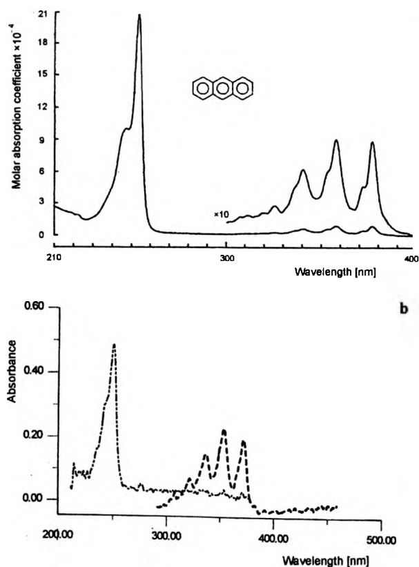
Fig. 2. Absorption spectrum of 0.73 mg/L anthracene in cyclohexane as obtained in reference [8] using Perkin–Elmer Model 555 instrument – a, absorption spectrum of the same concentration as in a obtained by the new system – b.
