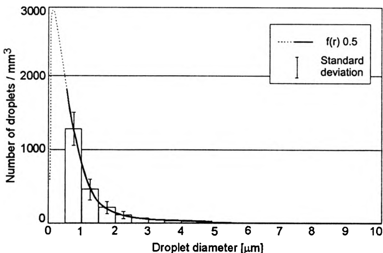
Fig. 1. Example of size distribution of oil droplets in water.
