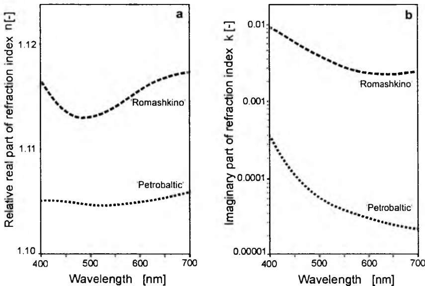
Fig. 2. Components of the complex light refraction index in oil: real part (a) in relation to the surrounding medium (sea water), and imaginary part (b).
