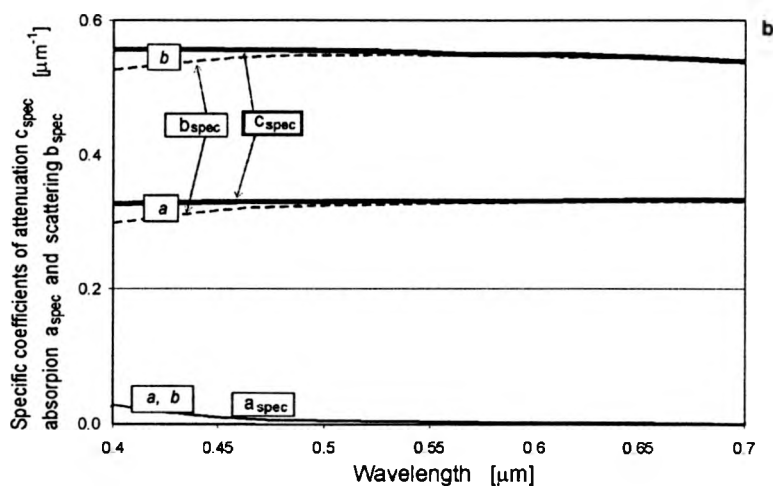
Fig. 6. Spectra of specific coefficients of light attenuation c_{\text{spec}} , absorption a_{\text{spec}} and scattering b_{\text{spec}} of emulsions of crude oil types Romashkino (a) and Petrobaltic (b) in one weak old emulsion a and two weak old emulsion b.
