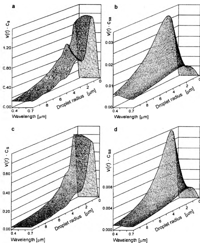
Fig. 4. Distributions of attenuation cross-sections (a) and (c) and absorption cross-sections (b) and (d) versus radius of suspension of crude oil type Romashkino after one week of aging (a) and (b), after two weeks of aging (c) and (d).
