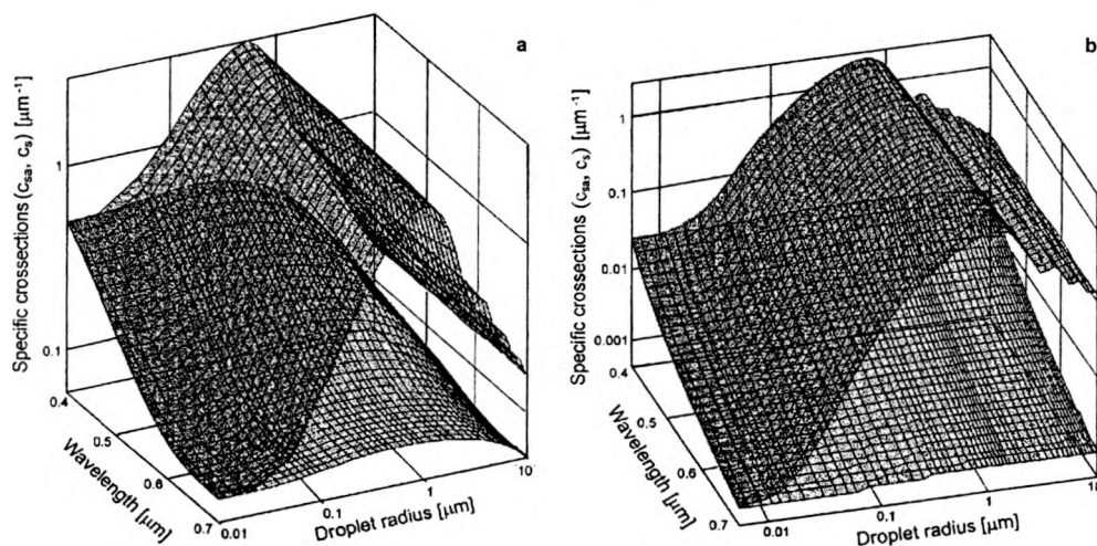
Fig. 3. Specific light attenuation cross-sections c_{sa} (left surfaces) and absorption c_a (right surfaces) for suspension of crude oil types Romashkino (a) and Petrobaltic (b).
