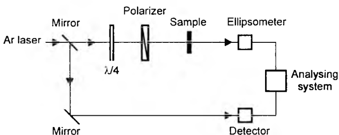
Fig. 1. Experimental setup ( \lambda/4 denotes the quarter-wave retarder).
