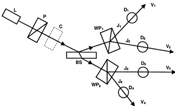
Fig. 2. General scheme of the Stokes ellipsometer. BS is the beam splitter, WP_1 and WP_2 are Wollaston prisms, D_1 , D_2 , D_3 and D_4 – linear photodetectors which produce electrical output signals V_1 , V_2 , V_3 and V_4 . L is the Argon laser light source, P – the polarizer and S – the sample. C is the quarter-wave retarder which is introduced during calibration of the instrument.
