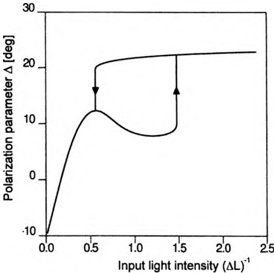
Fig. 4. Theoretical dependence of phase difference \Delta (in degrees) between two linear components of polarization of the output light as a function of the input light intensity, for the case of electric vector \mathbf{E} of input light perpendicular to the director \mathbf{n} of the liquid crystal. Light intensity is in arbitrary units (\Gamma L)^{-1} .
