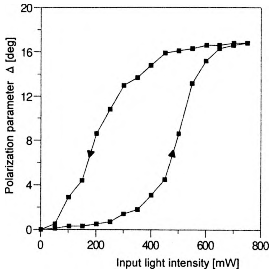
Fig. 3. Phase difference \Delta (in degrees) between two linear components of polarization of the output light as a function of the input light intensity, measured for the electric vector \mathbf{E} of input light perpendicular to the director \mathbf{n} of the liquid crystal.
