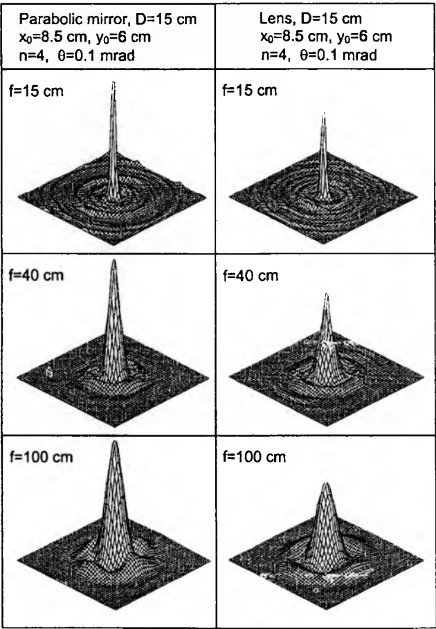
Fig. 3. Light intensity distributions in the focal planes of the parabolic mirror and the lens of various focal length. The peak intensities in each column are normalized to the same value.
