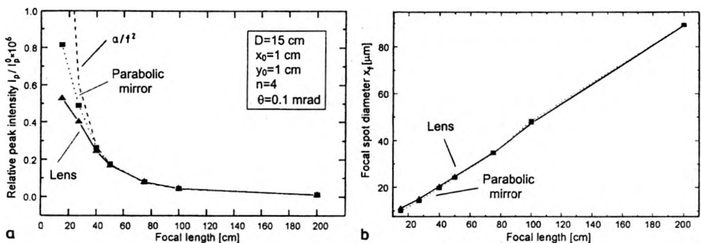
Fig. 2. Relative peak intensity of light after focusing (a) and the focal spot diameter (b) as a function of the focal length for the case of small-aperture beam.
