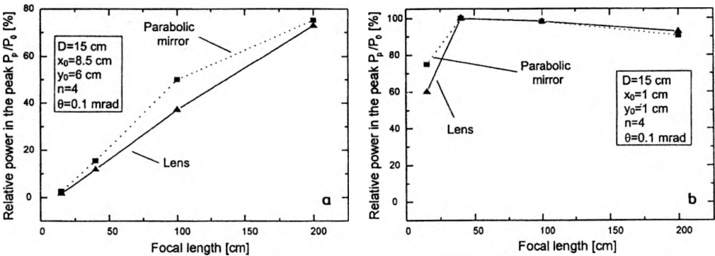
Fig. 4. Relative power stored in the central peak of the focal intensity distribution as a function of the focal length for the cases of large-aperture (a) and small-aperture (b) beams.
