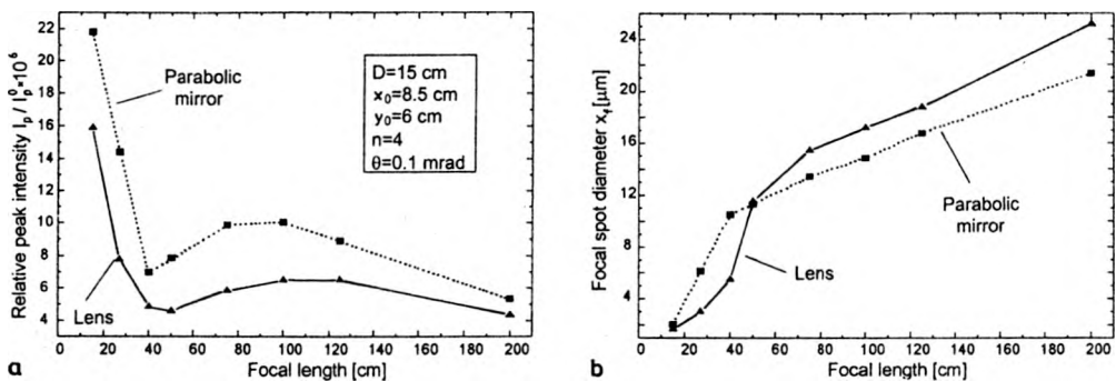
Fig. 1. Relative peak intensity of light after focusing (a) and the focal spot diameter (b) as a function of the focal length for the case of large-aperture beam.
