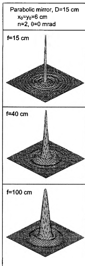
Fig. 7. Light intensity distributions in the focal plane of parabolic mirror of various focal length for the case of large-aperture Gaussian beam with plane wave front. The peak intensities are normalized to the same value.
