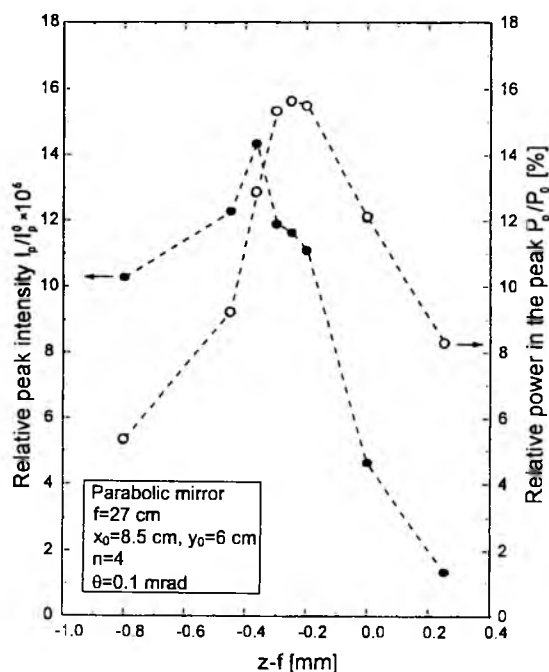
Fig. 5. Relative peak intensity of light in the plane z and relative power stored in the central peak as a function of the distance of the plane z from the nominal focal plane z = f .
