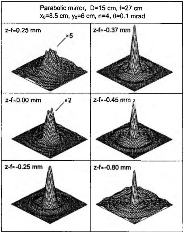
Fig. 6. Light intensity distributions in the plane z for various distances of the plane z from the nominal focal plane z = f .
