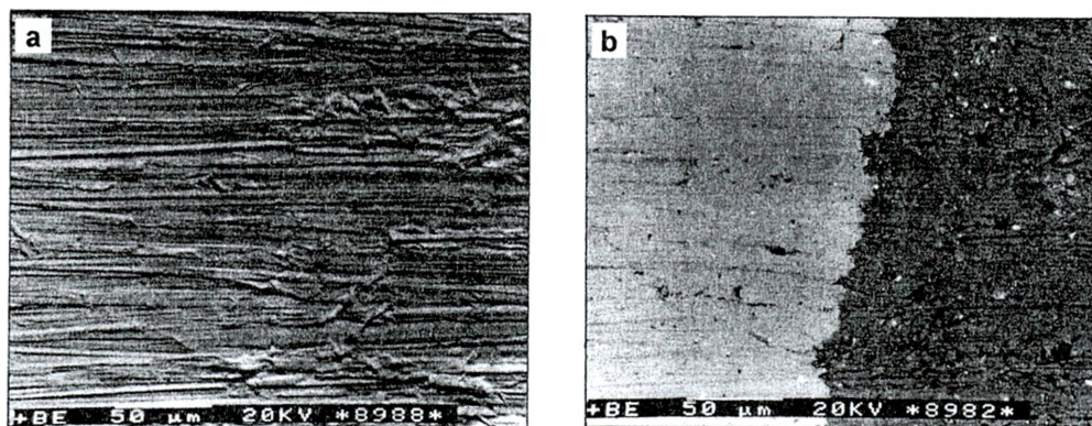
Fig. 3. Scanning electron micrographs of Mo–Cu weld interface: a – in TPO mode (D1–D2), b – in COMPO mode (D3+D4).
