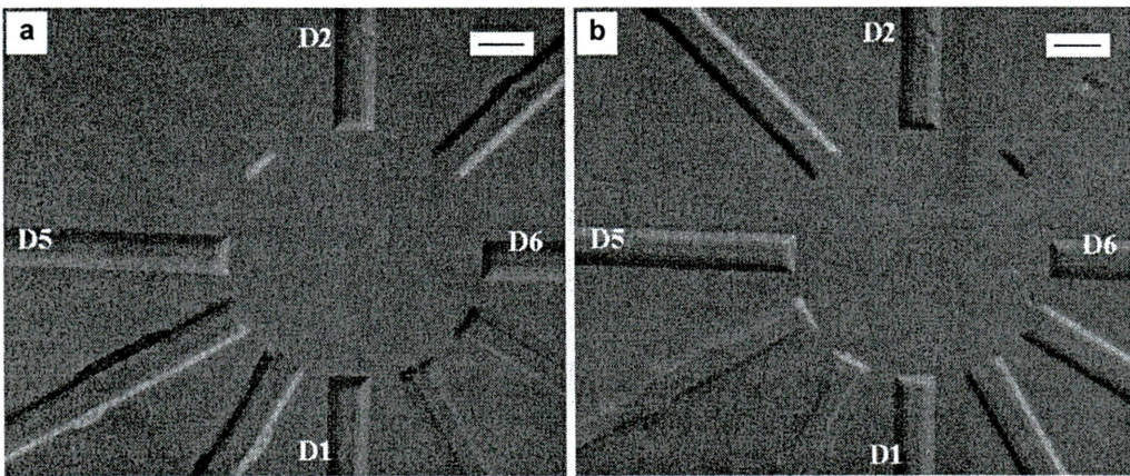
Fig. 6. Surface digital images with radially located grooves in case where: a – TOPO mode is produced according to the algorithm ( D2-D1 )+( D6-D5 ), b – TOPO mode is produced according to the algorithm ( D1-D2 )+( D6-D5 ) (bar = 50 \mu\text{m} ).
