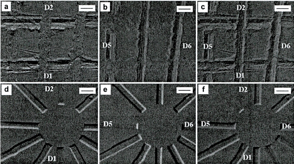
Fig. 5. Surface digital images with crossing scratches and radial grooves: a, d – images obtained as a result of BSE signal subtraction from detectors ( D2-D1 ), b, e – as above, but as a result of signal subtraction from detectors ( D6-D5 ), c, f – as above, but in effect of addition of signal difference ( D2-D1 )+( D6-D5 ). Location of detectors has been marked on the particular images (bar = 75 \mu\text{m} ).
