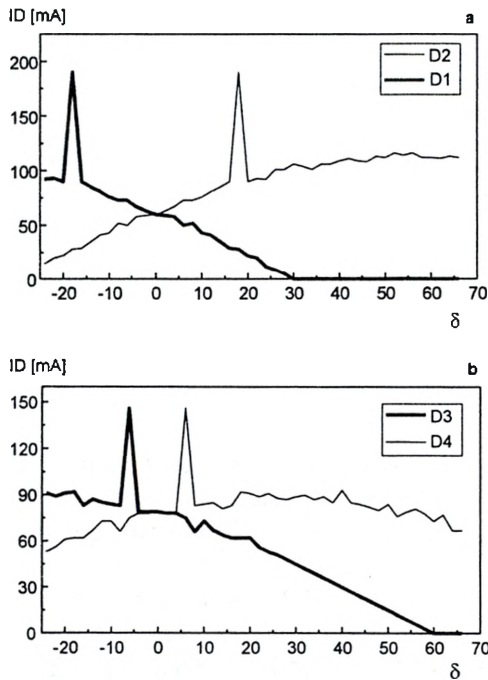
Fig. 8. Dependence of BSE current ID on the surface inclination angle \delta of Au sample in the case of detectors: a — D1, D2, b — D3, D4.
