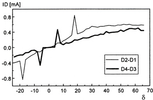
Fig. 9. Dependence of detector current ID on the surface inclination angle \delta of Au specimen in the case of TOPO mode realization as (D2 - D1) and (D4 - D3) .
