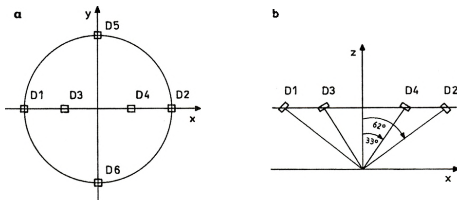
Fig. 1. Arrangement of detectors in relation to the coordinate system x-y-z: a — top view, b — detection angles quantity.
