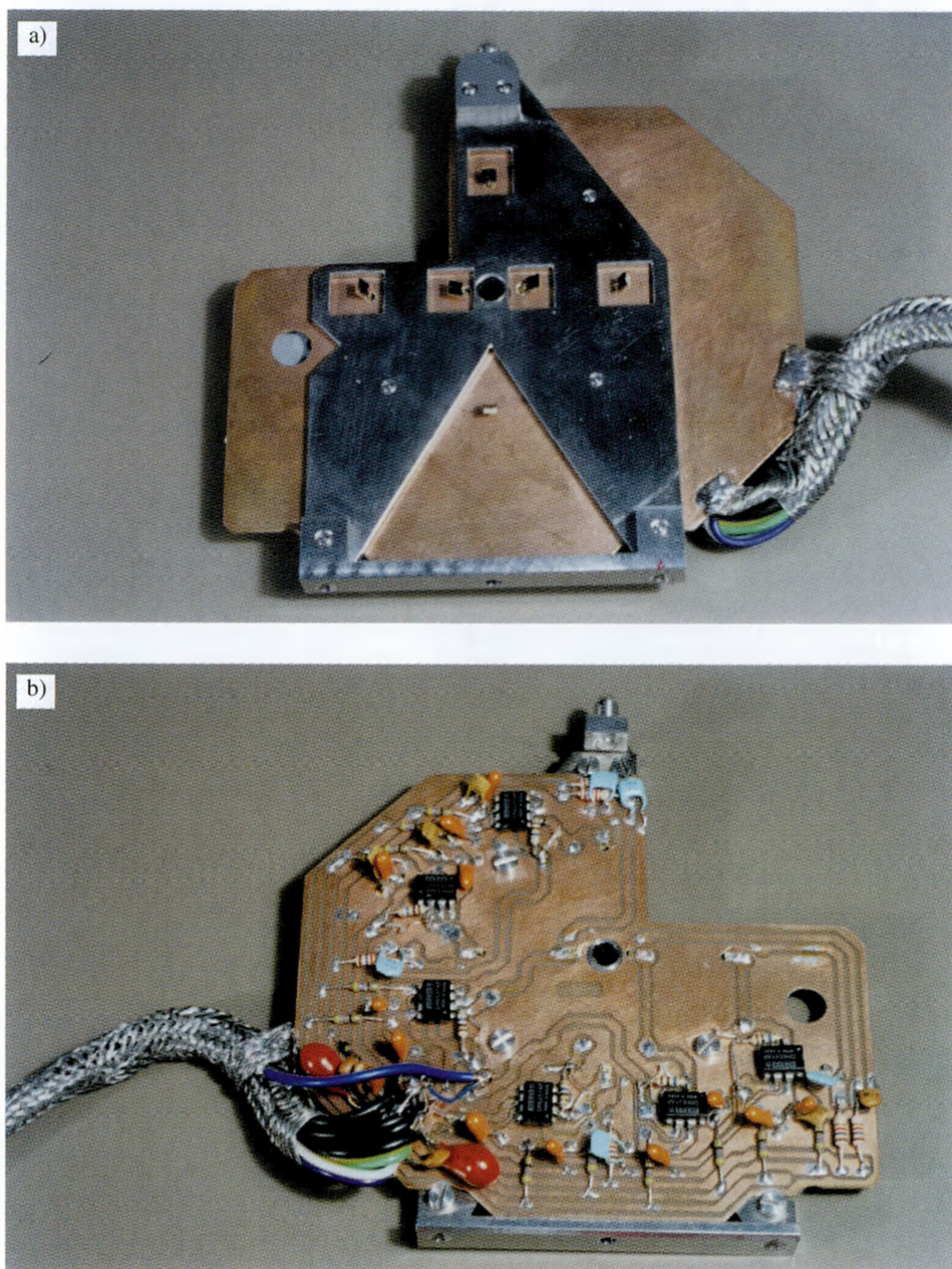
Fig. 2. The detector system view from: a) the p-i-n diodes side; b) the preamplifiers side
