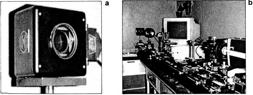
Fig. 2. RWD element (a) and lens-RWD-based feature extractor (b) [7].
