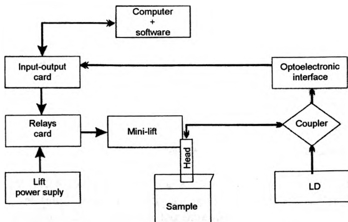
Fig. 1. Block diagram of automatic sensor.
