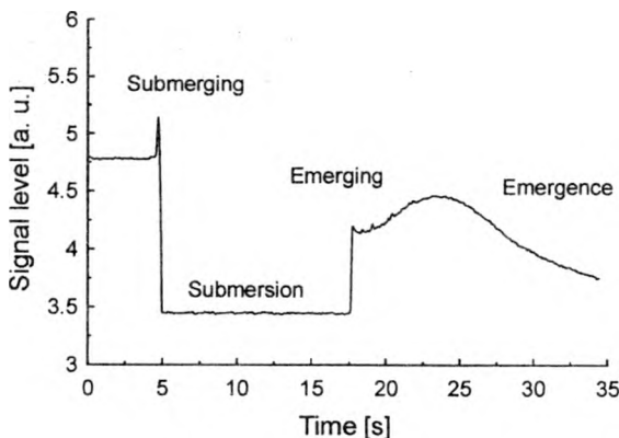
Fig. 2. Full measuring cycle in the time domain for edible oil sample.
