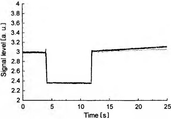
Fig. 8. Measuring cycles for alcohol sample.
