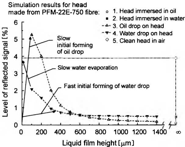
Fig. 5. Slow variation and constant reflected signals coming from the head.
