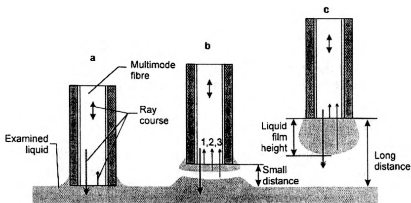
Fig. 4. Emerging of the sensor from the liquid under examination.
