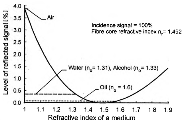
Fig. 3. Reflected signal from a submersed head.
