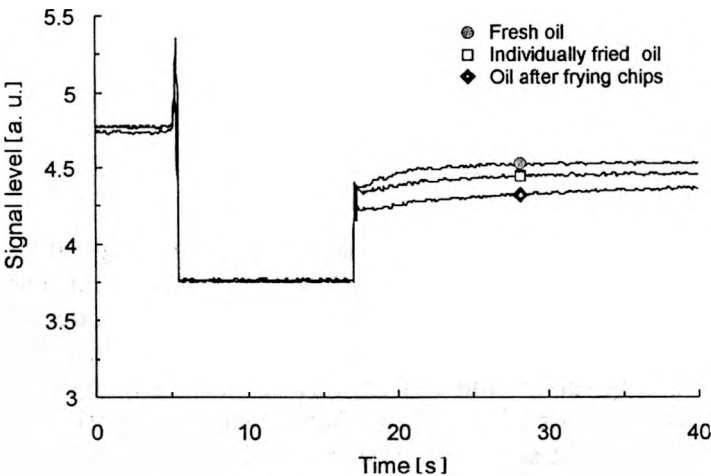
Fig. 9. Measuring cycles for the head immersed 1 mm in oil.
