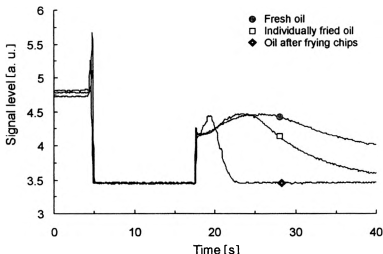
Fig. 10. Measuring cycles for head immersed 10 mm in oil.
