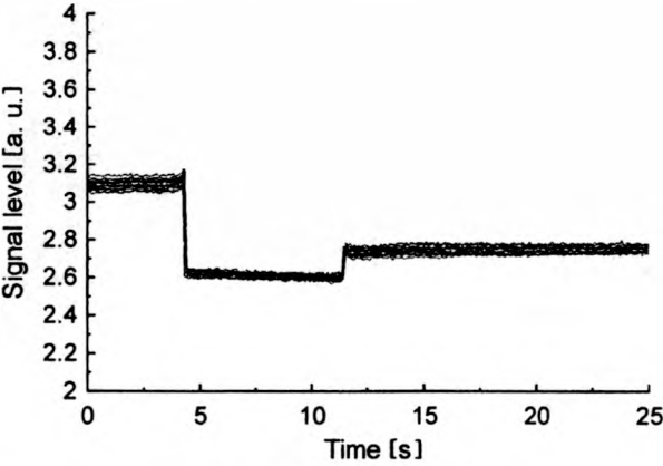
Fig. 6. Measuring cycles for water sample.
