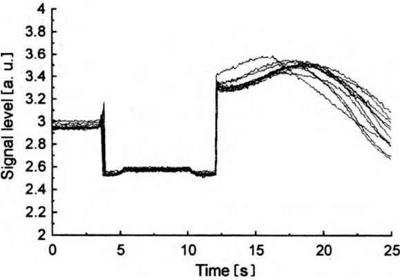
Fig. 7. Measuring cycles for eatable oil sample.
