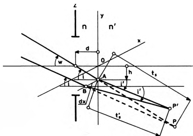
Fig. 4. Astigmatic light pencil in sagittal cross-section.
