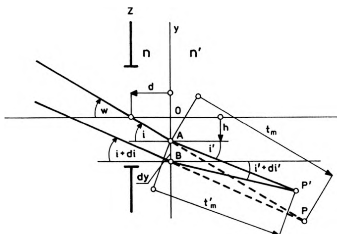
Fig. 3. Astigmatic light pencil in meridional cross-section.
