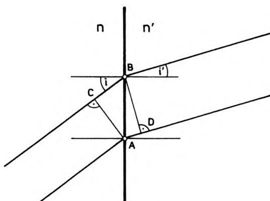
Fig. 1. Deviation of light rays on hybrid surface.
