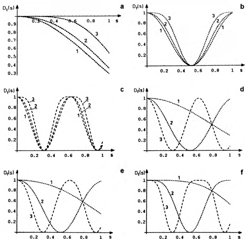
Fig. 2. Effect of amplitude apodisation t(r) = \cos^2(Nr) on the contrast of image of the amplitude object test for: a - N = 1 , m = 0 (1), m = 0.5 (2), m = 1.0 (3), b - N = 3 , m = 0 (1), m = 0.5 (2), m = 1.0 (3), c - N = 5 , m = 0 (1), m = 0.5 (2), m = 1.0 (3), d - m = 0 , N = 1 (1), N = 3 (2), N = 5 (3), e - m = 0.5 , N = 1 (1), N = 3 (2), N = 5 (3), f - m = 1.0 , N = 1 (1), N = 3 (2), N = 5 (3).
