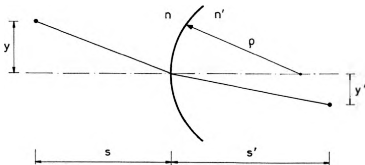
Fig. 5. Imaging geometry by a single spherical surface.
