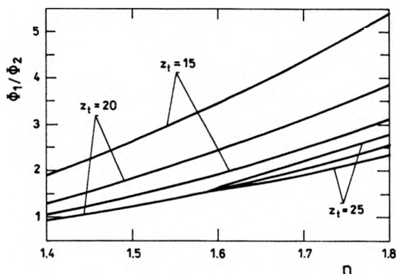
Fig. 11. Dependence parameter \phi_1 = \phi_1/\phi describing the lens shape assuring correction of astigmatism on index of refraction n for a few typical values of the input pupil outset z_1 and focusing power \Phi = +10 D and object at infinity.
