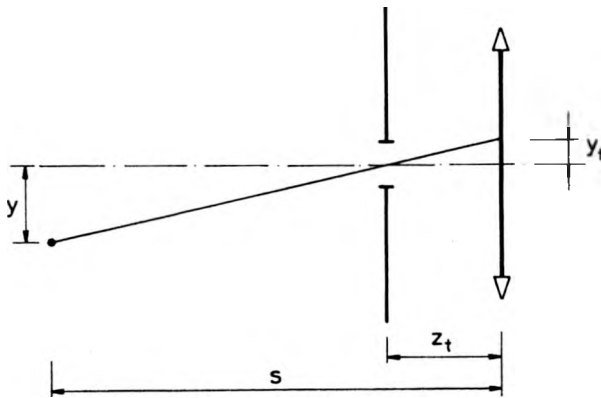
Fig. 9. Lens with the shifted input pupil — geometry relations.
