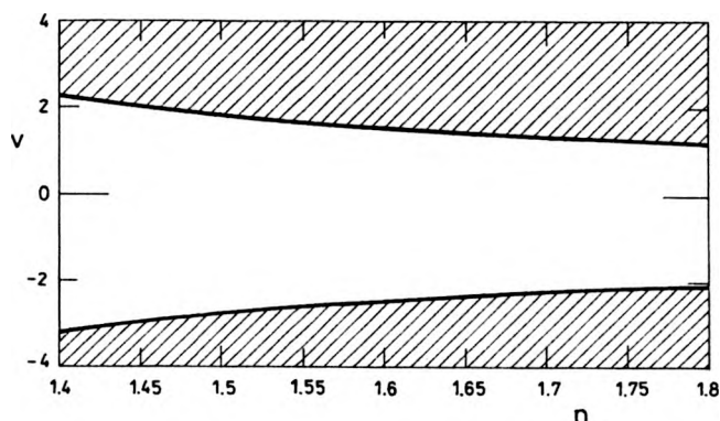
Fig. 6. Range of parameter v describing object distance for which the correction of spherical aberration is possible as a function of values of refractive index n .
