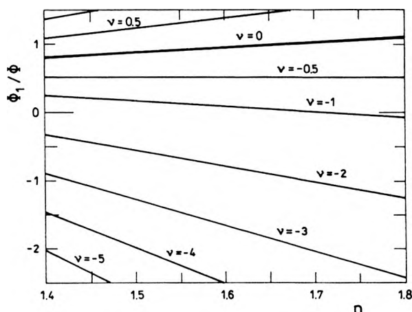
Fig. 7. Values of parameter \phi_1 = \Phi_1/\Phi describing the shape of the lens minimised spherical aberration versus the refractive index n for different object locations: v = 0 – object at infinity, v < 0 – object in front of the lens (real), v > 0 – object behind the lens (imaginary).
