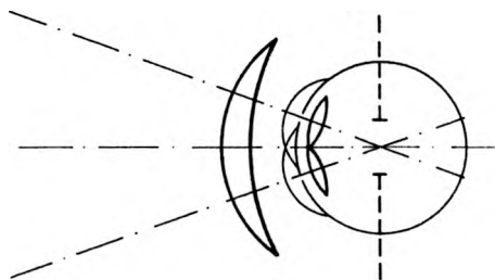
Fig. 2. Aperture diaphragm in the optical system composed of the eye and spectacle lens.
