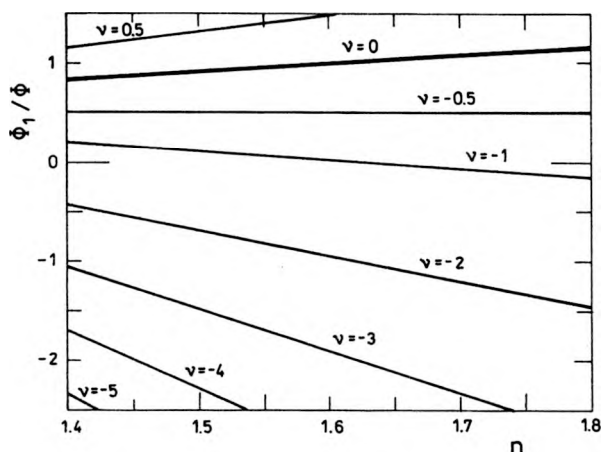
Fig. 8. Values of parameter \varphi_1 = \Phi_1/\Phi determining the shape of coma-free lens as a function of value of refractive index n for different object locations: v = 0 — object at infinity, v < 0 — object in front of the lens (real), v > 0 — object behind the lens (imaginary).
