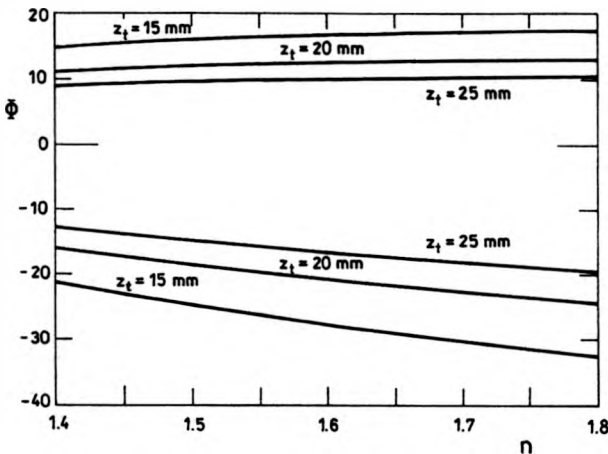
Fig. 10. Range of total focusing power \Phi , where the correction of astigmatism is possible versus refractive index n for selected values of input pupil shift z_t .
