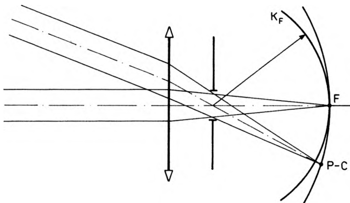
Fig. 4. Positive lens with shifted pupil and its Petzval-Coddington surface (P-C) and focal sphere K_F .
