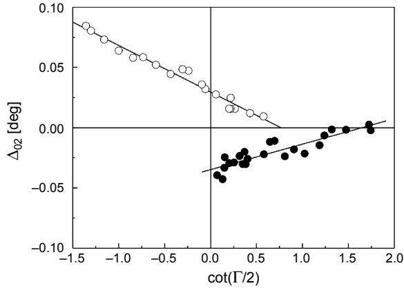
Fig. 2. Plots of the parameter \Delta_{02} versus \cot(\Gamma/2) for the CGG crystals. The two plots correspond to alternative specimen orientations as obtained before (○) and after (●) rotating the specimen by 90^\circ around the light beam direction. Solid lines represent the best fit to Eq. (2).
