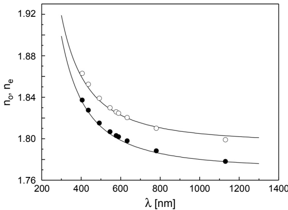
Fig. 3. Dispersions of the ordinary (●) and extraordinary (○) refractive indices calculated for the CGG crystals: lines represent the experimental results [1, 2].
