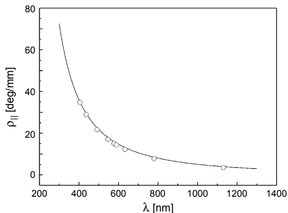
Fig. 4. Calculated dispersion of the absolute value of \rho_{||} parameter for the CGG crystals: line represents the experimental results [1, 2].
