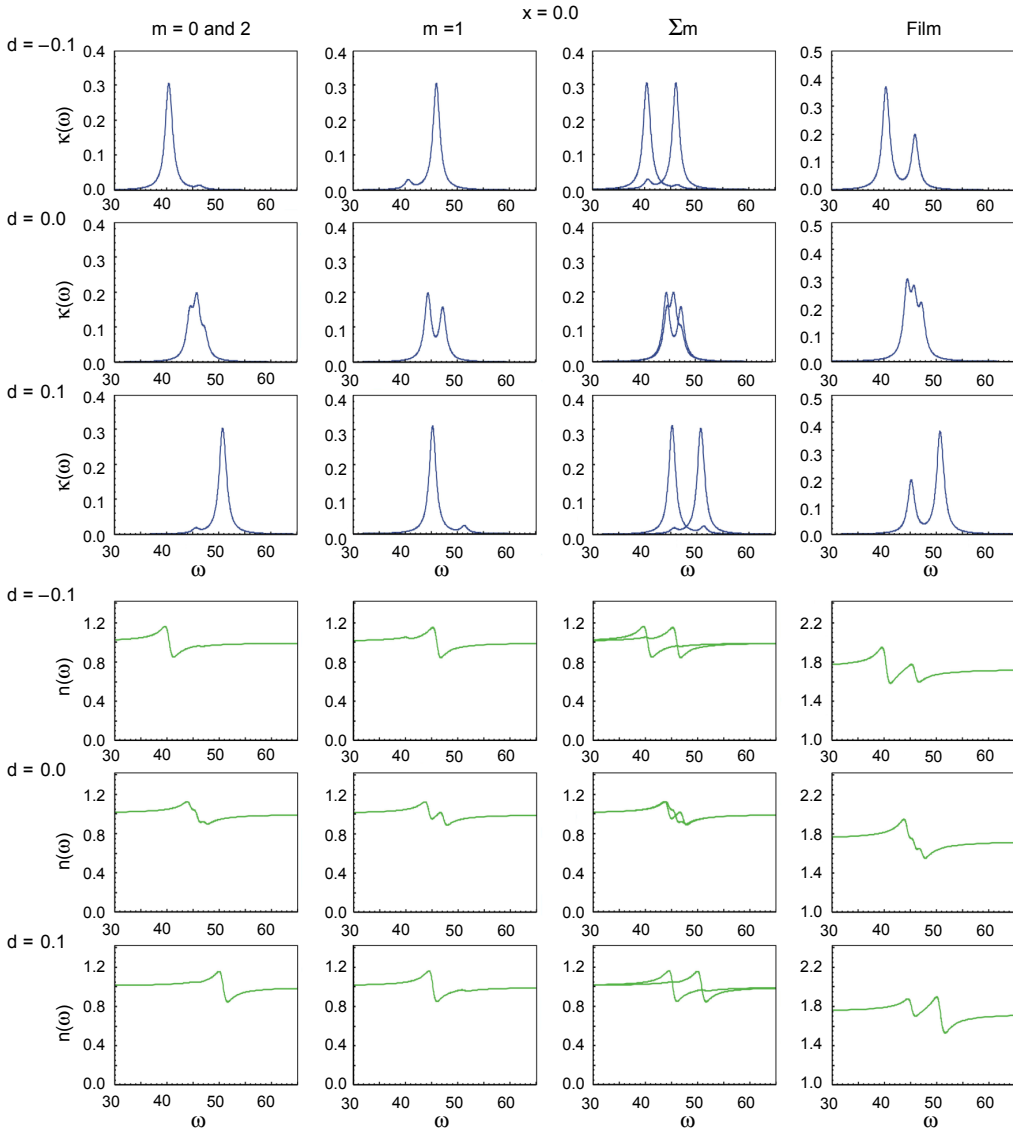
Fig. 2. Relative dynamical absorption and refraction indices of symmetrical perturbed two-layered film (see text for explanation).
