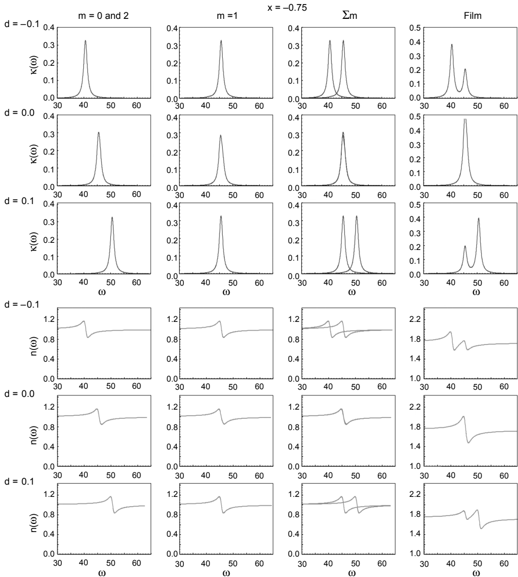
Fig. 1. Relative dynamical absorption and refractive indices of symmetrical perturbed two-layered film (see text for explanation).
