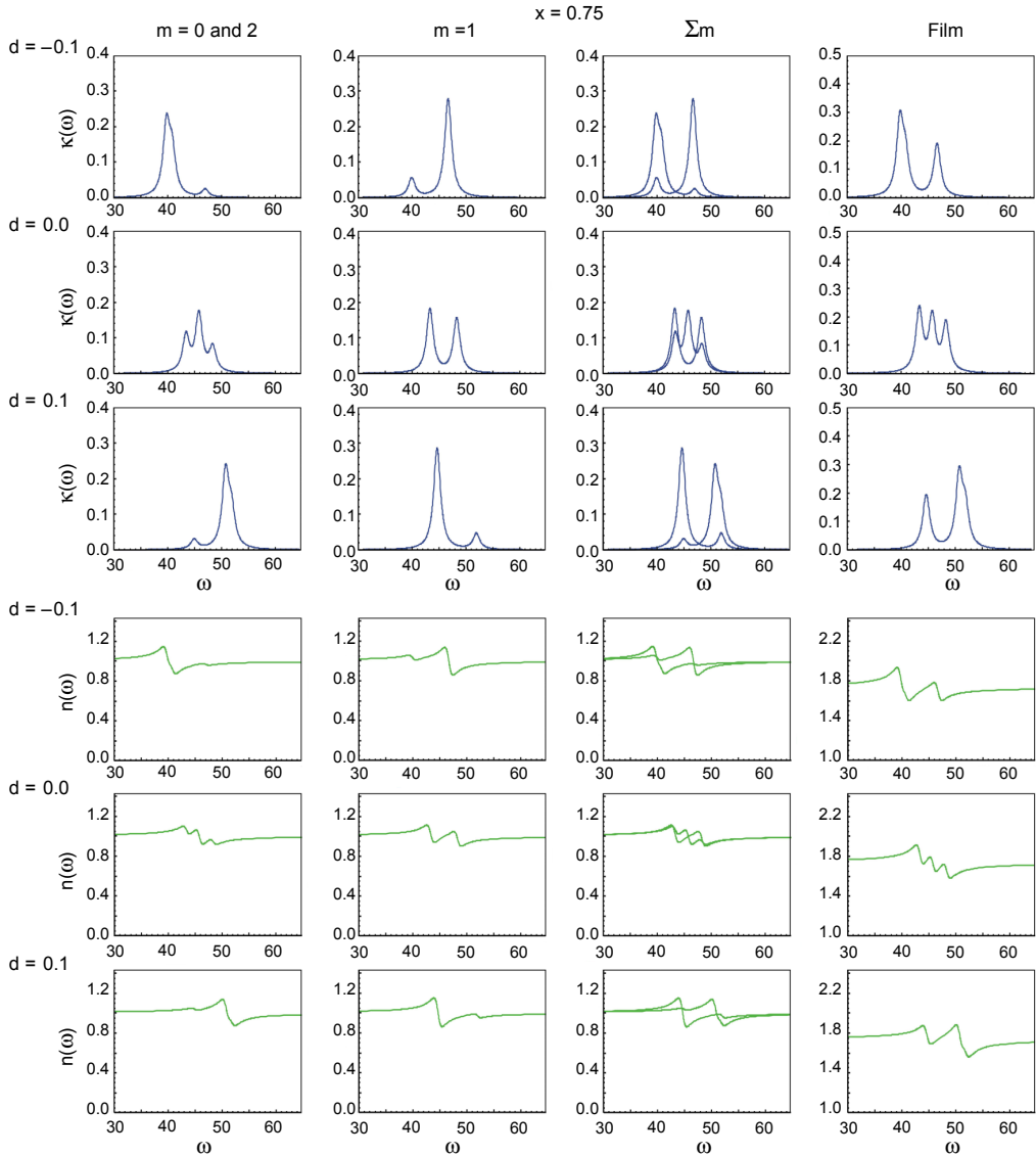
Fig. 3. Relative dynamical absorption and refractive indices of symmetrical perturbed two-layered film (see text for explanation).
