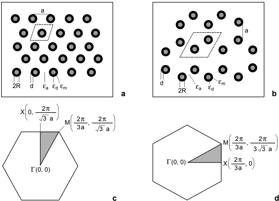
Fig. 1. Schematic structures of 2D MDPCs which contain dielectric central rods with metallic outer shell. Triangular structure (a), honeycomb structure (b), irreducible Brillouin zone of the triangular structure (c), and irreducible Brillouin zone of the honeycomb structure (d). Both structures are arranged in air background. The structure of a unit cell is indicated by a dashed line. The black, gray and white area represent metal, dielectric and air, respectively.
