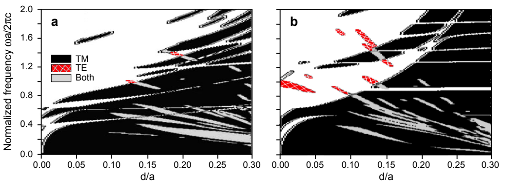
Fig. 6. Gap maps for 2D MDPCs in triangular (a) and honeycomb (b) structure. Radius of an alumina rod is R = 0.2a , where a is 500 nm, dielectric constant of an alumina rod and air background are \epsilon_d = 8.9 and \epsilon_a = 1 , respectively.
