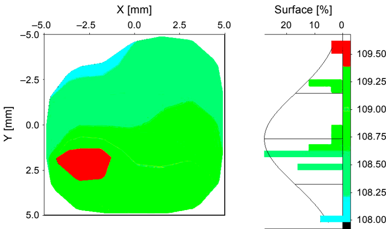
Fig. 9. The thickness distribution map of a sample C deposited with 1030 cycles at 300°C substrate temperature.
