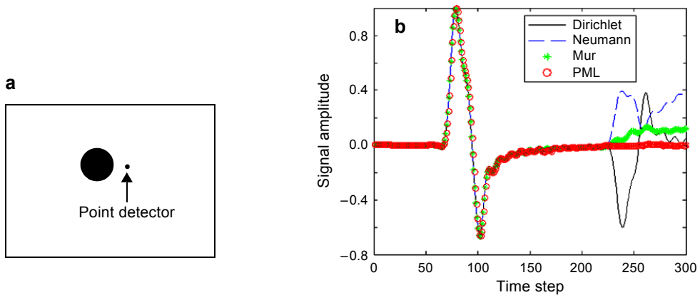
Fig. 7. Comparison of the effect of different boundary conditions on photoacoustic signal. Circular object within a rectangular domain and a point detector at the right side (a), and photoacoustic signals detected by a point detector (b).
