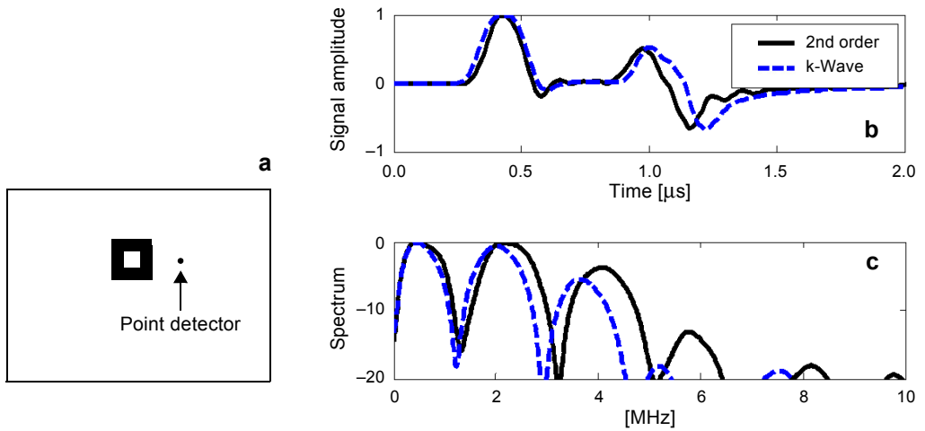
Fig. 5. Squared donut-shaped object and a point detector (a). Time-domain signal of a point detector at 1 mm from the origin (b) and its spectrum (c).
