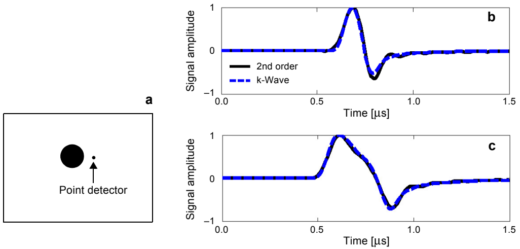
Fig. 2. Circular object within a rectangular domain and a point detector at the right side (a). Time-domain signal of 200- \mu\text{m} (b) and 500- \mu\text{m} (c) objects.
