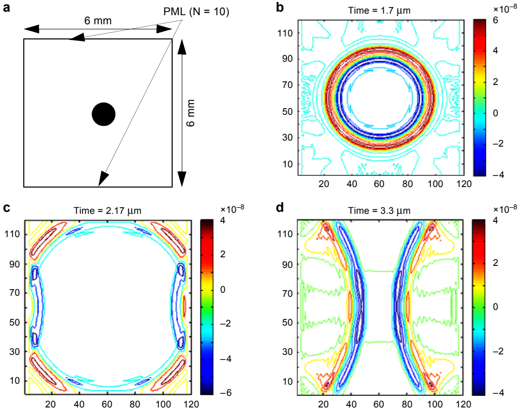
Fig. 6. Effect of PML boundary condition for a circular object in 6 \times 6 mm domain in which the upper and lower boundary condition is PML with 10 layers and the other is Dirichlet boundary condition (a). Propagating photoacoustic waves after 1.7 \mu\text{s} (b), 2.17 \mu\text{s} (c) and 3.3 \mu\text{s} (d).
