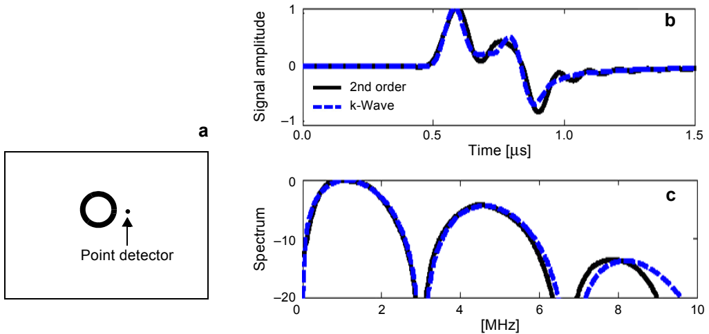
Fig. 3. Donut-shaped object and a point detector (a). Time-domain signal of a point detector at 1 mm from origin (b) and its spectrum (c).
