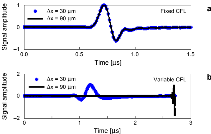
Fig. 1. Solution for a 200- \mu\text{m} object with two mesh sizes and fixed \text{CFL} = 0.3 – a , and with two mesh size and variable \text{CFL} of 0.538 (black line) and 0.194 (dotted line) – b .
