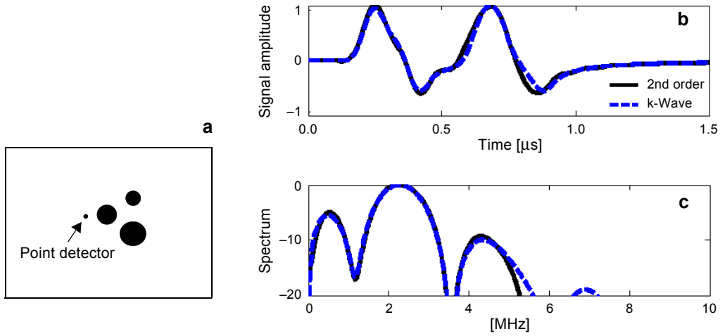
Fig. 4. Three 200-, 300- and 500- \mu\text{m} circular objects illuminated in a rectangular domain and a point detector (a). Time-domain signal (b) and its spectrum (c).
