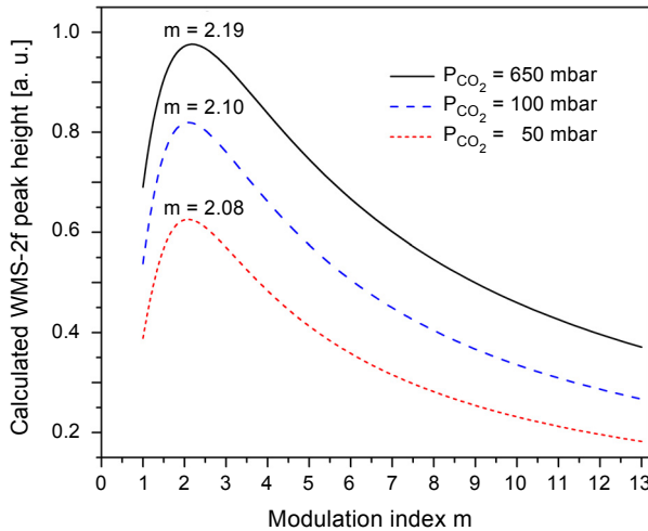
Fig. 5. Variation of WMS-2f peak height with modulation index for three CO 2 pressures. Simulation is performed at room temperature for R(22) CO 2 absorption line centered at 6363.727 cm -1 . Modulation frequency is assumed 300 Hz.
