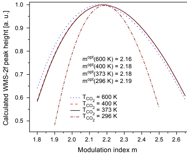
Fig. 4. Variation of WMS-2f peak height with modulation index for four distinctive gas temperatures. Simulation is performed for R(22) CO 2 absorption line centered at 6363.727 cm -1 . Gas pressure is taken fixed at 650 mbar and modulation frequency is assumed 300 Hz.
