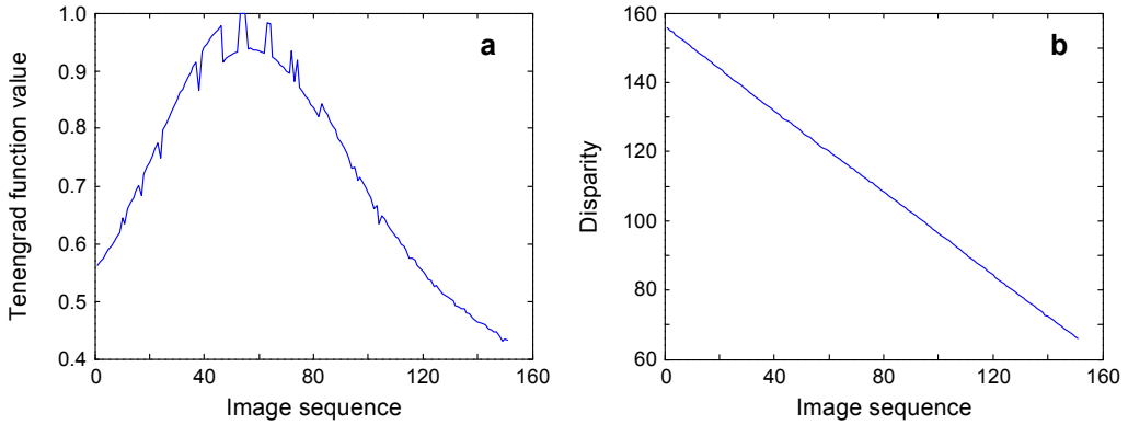
Fig. 3. Tenengrad function values of the left views of calibrated stereomicroscopic image sequence (a); disparities of calibrated stereomicroscopic image sequence (b).
