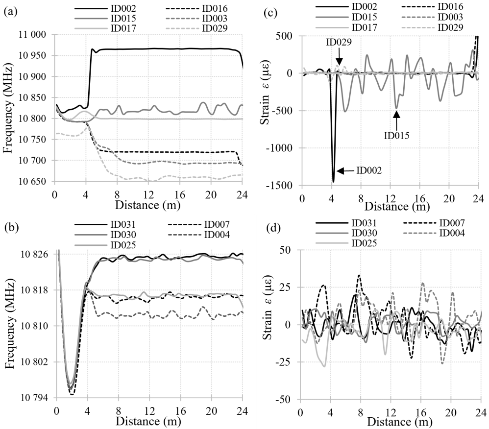
Fig. 3. Baseline (a, b) and corresponding strain (c, d) measurements results for representative ITU-T compliant optical fibers.
