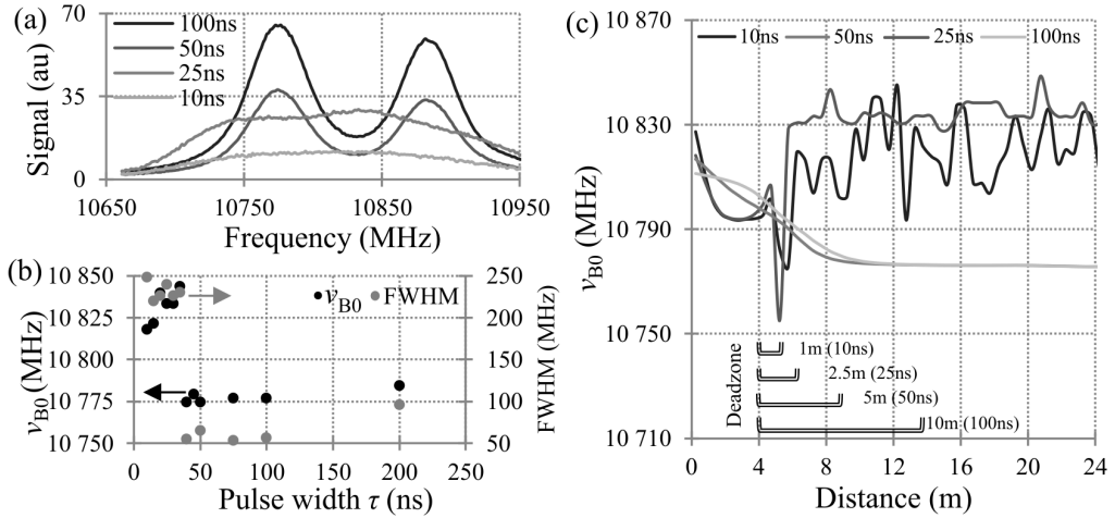
Fig. 4. Influence of optical laser pulse width on: Brillouin spectral response (a), main frequency shift and FWHM (b), and baseline stability (c), for ID015 Corning SMF-28e+ optical fiber.
