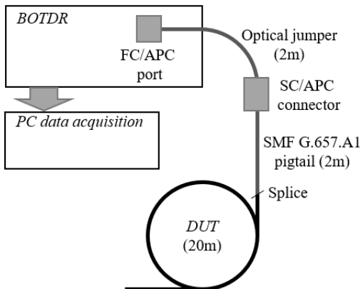
Fig. 1. Measurement system block scheme.
