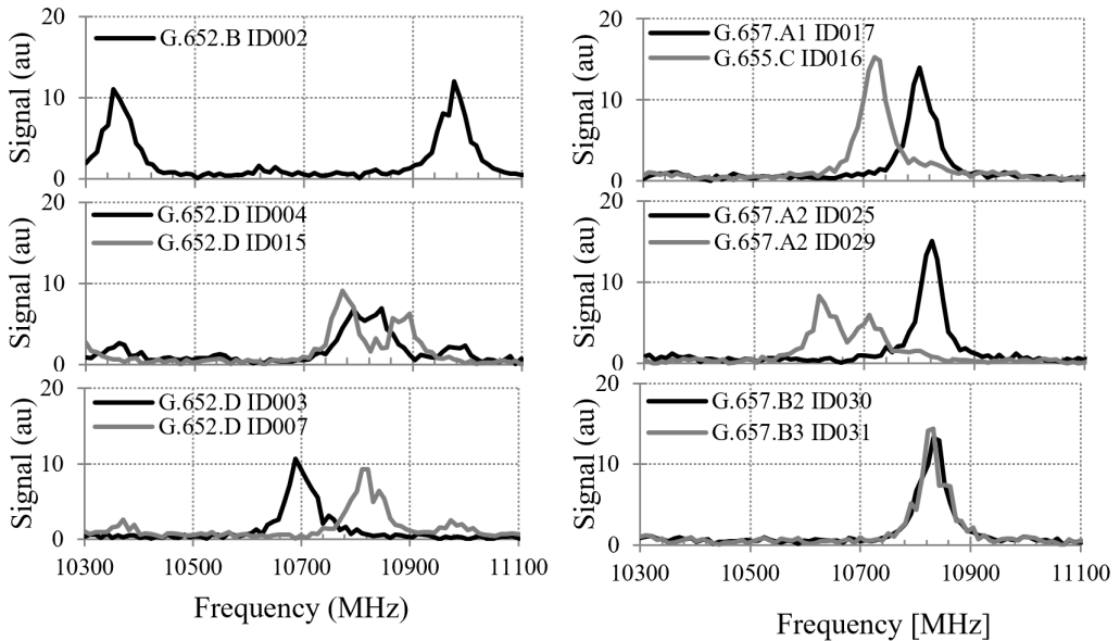
Fig. 2. Rough spectral characteristics of several optical fibers.
