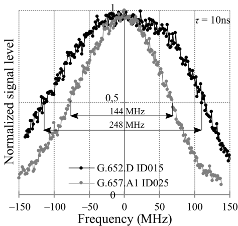
Fig. 6. Comparison of two extreme cases of FWHM from all measured optical fibers.
