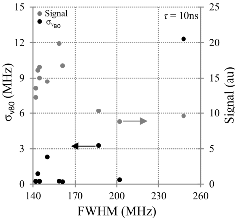
Fig. 5. Dependence of FWHM on: Brillouin frequency standard variation and signal level, based on measured optical fibers from representative group.
